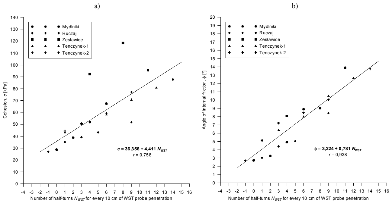
Fig. 5. Relation between cohesion and angle of internal friction and half-turn number N_{WST} (a) cohesion c , (b) angle of internal friction \phi Mydlniki [1], Ruczaj [1], Zesławice [1], Tenczynek-1 [22]
