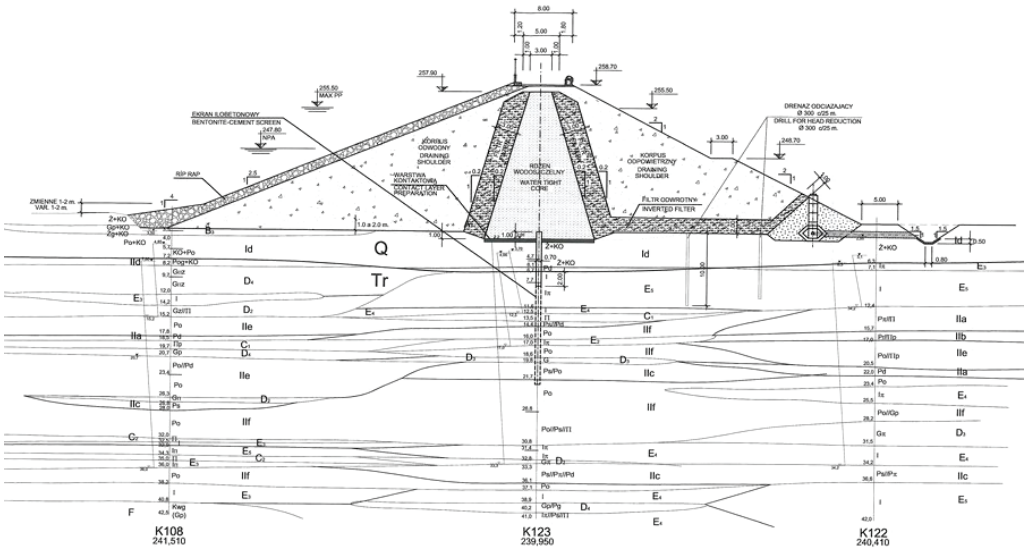
Fig. 3. Cross-section through the front dam with bedrock geology according to [1]
