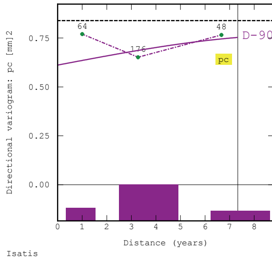
Fig. 3. Directional variogram of total displacements p_c \text{ [mm]}^2 for the Opatowice weir along the time Z-axis approximated by the theoretical model from the years of observation (1986–1998)
