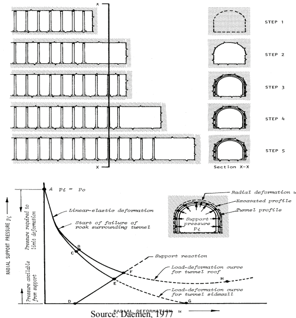
Fig. 7. Hypothetical drilling and blasting tunnel excavation with steel set support and load deformation curves
