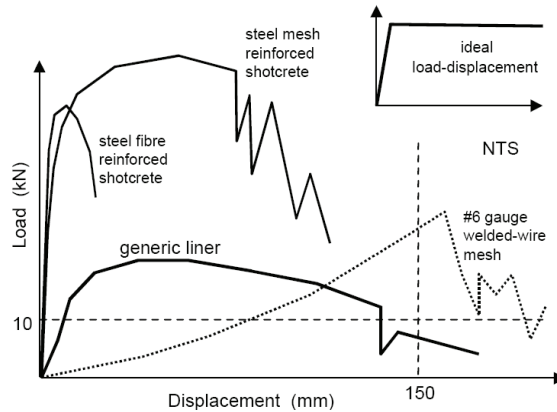
Fig. 15. Schematic load displacement curves of areal supports
