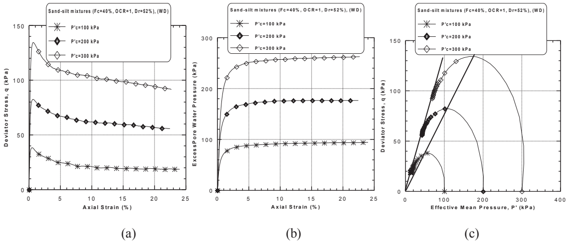
Figure 12: Undrained monotonic response of wet deposited sand-silt mixtures ( F_c = 40\% , OCR = 1 , D_r = 52\% ): (a) deviator stress versus axial strain, (b) excess pore water pressure versus axial strain and (c) stress path diagram.
