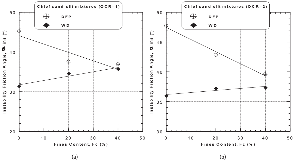
Figure 16: Instability friction angles versus fines content of sand–silt mixtures ( D_r = 52\% ): (a) OCR = 1 and (b) OCR = 2.
