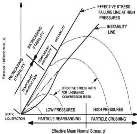
Figure 1: Determination of the instability line (Yamamuro and Lade, 1997).
