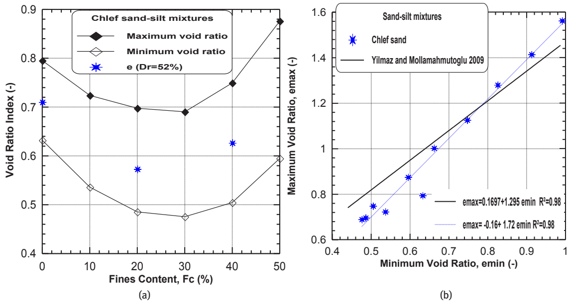
Figure 4: Void ratios index of tested soils. (a) Void ratio index versus fines content and (b) maximum void ratio versus minimum void ratio.
