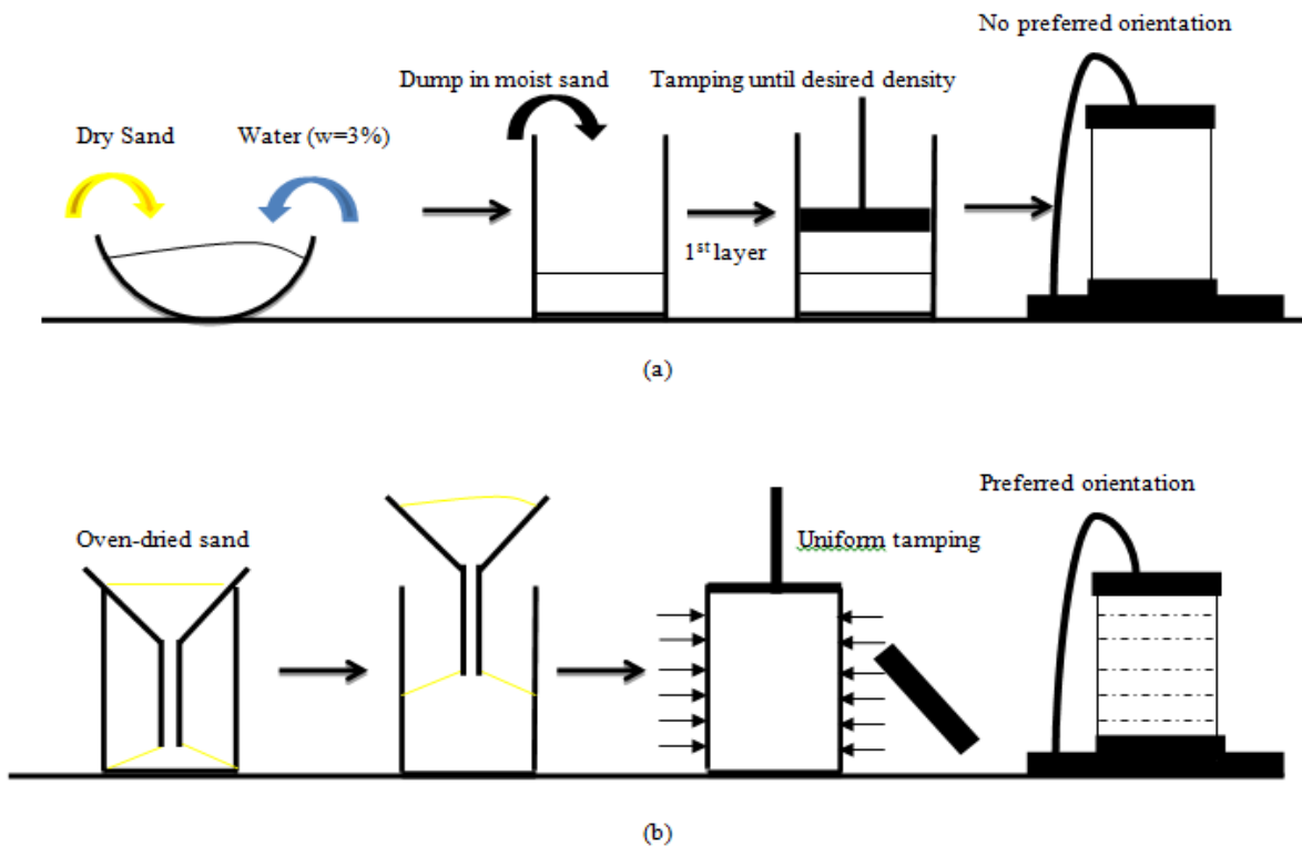
Figure 5: Schematic illustration of sample preparation; (a) wet deposition and (b) dry funnel pluviation.
