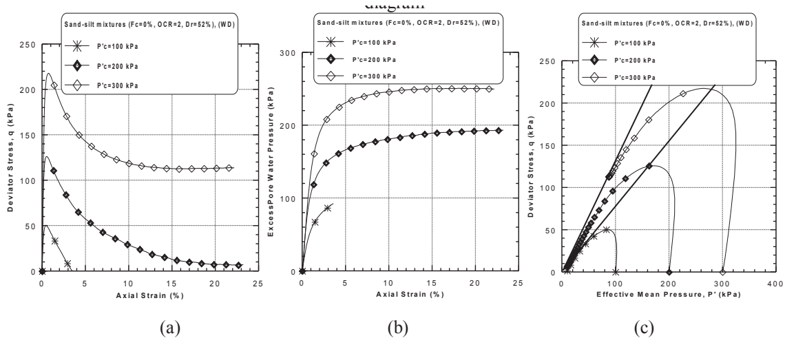
Figure 13: Undrained monotonic response of wet deposited sand-silt mixtures ( F_c = 0\% , OCR = 2 , D_r = 52\% ): (a) deviator stress versus axial strain, (b) excess pore water pressure versus axial strain and (c) stress path diagram.
