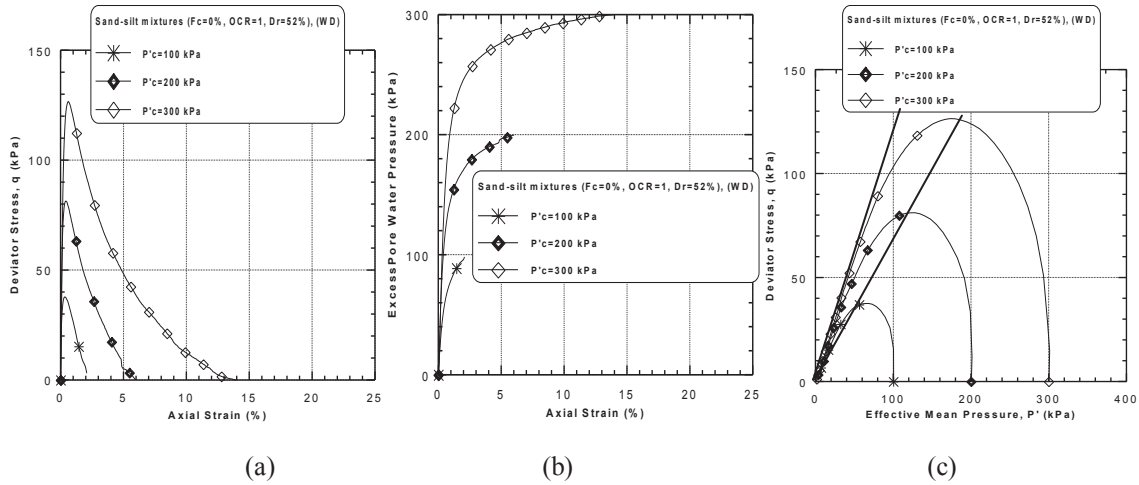
Figure 11: Undrained monotonic response of wet deposited sand-silt mixtures ( F_c = 0\% , OCR = 1 , D_r = 52\% ): (a) deviator stress versus axial strain, (b) excess pore water pressure versus axial strain and (c) stress path diagram.
