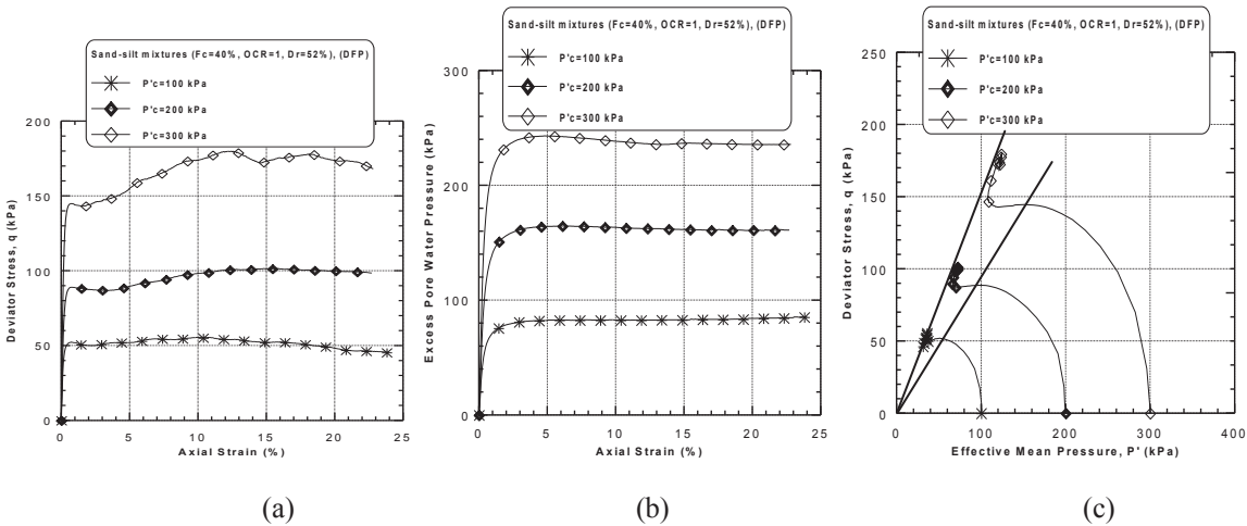
Figure 8: Undrained monotonic response of dry funnel pluviated sand-silt mixtures ( F_c = 40\% , OCR = 1 , D_r = 52\% ): (a) deviator stress versus axial strain, (b) excess pore water pressure versus axial strain and (c) stress path diagram.
