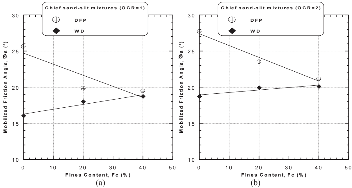
Figure 22: Mobilised friction angles versus fines content of sand-silt mixtures ( D_f = 52\% ): (a) OCR = 1 and (b) OCR = 2.
