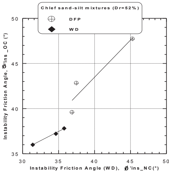
Figure 18: Overconsolidated instability friction angle versus normally consolidated friction angle of sand-silt mixtures ( D_r = 52\% ).
