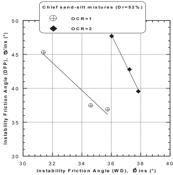
Figure 17: DFP instability friction angle versus WD friction angle of Chlef sand-silt mixtures ( D_r = 52\% ).
