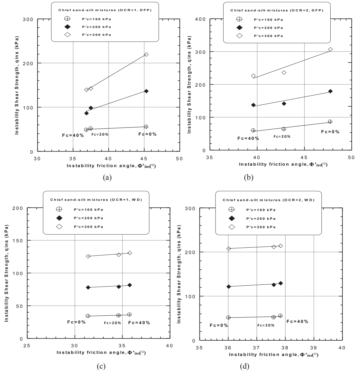
Figure 21: Instability shear strength versus the instability friction angle of sand-silt mixtures ( D_r = 52\% ): (a) OCR = 1, DFP; (b) OCR = 2, DFP; (c) OCR = 1, WD; (d) OCR = 2, WD.
