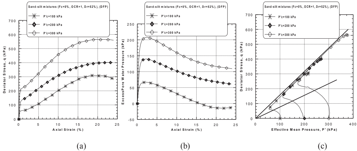
Figure 7: Undrained monotonic response of dry funnel pluviated sand-silt mixtures ( F_c = 0\% , OCR = 1 , D_r = 52\% ): (a) deviator stress versus axial strain, (b) excess pore water pressure versus axial strain and (c) stress path diagram.
