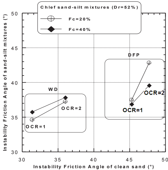
Figure 19: Instability friction angle of sand–silt mixtures versus instability friction angle of sand ( D_r = 52\% ).
