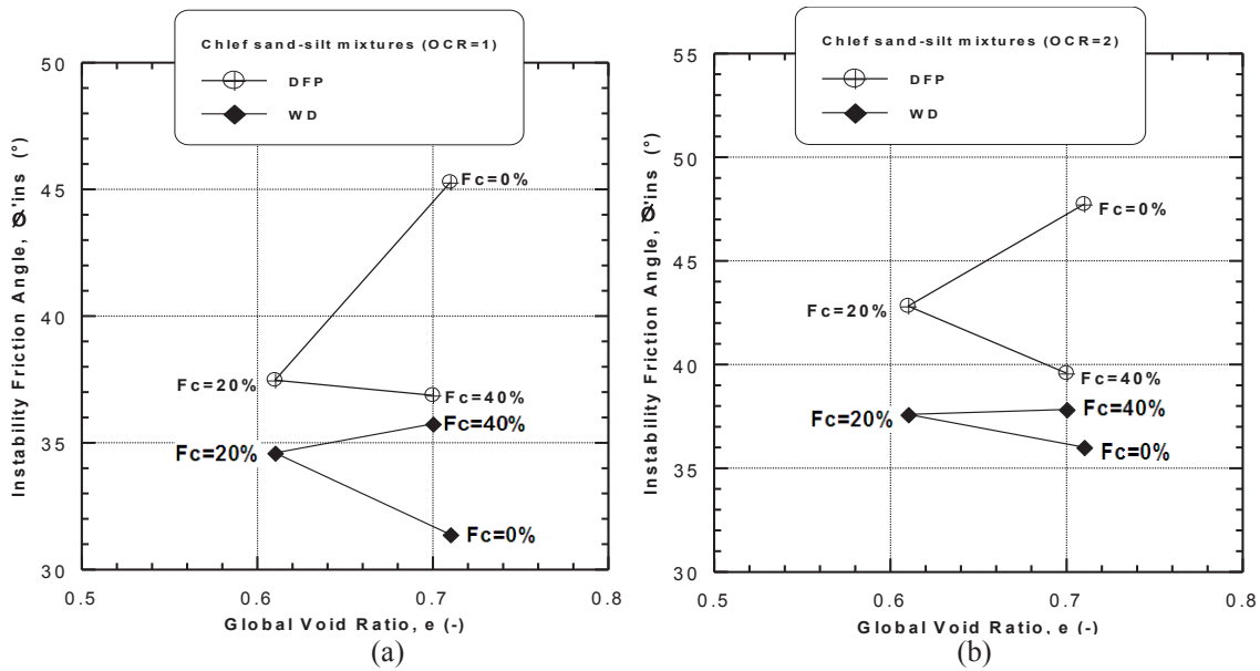
Figure 24: Instability friction angles versus global void ratio: (a) OCR = 1 and (b) OCR = 2.
