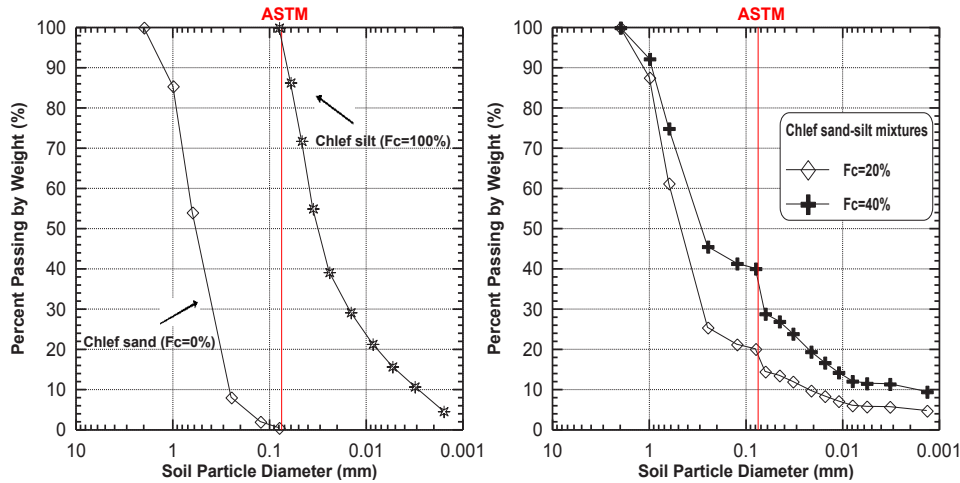
Figure 3: Grain size distribution curves of tested soils.
