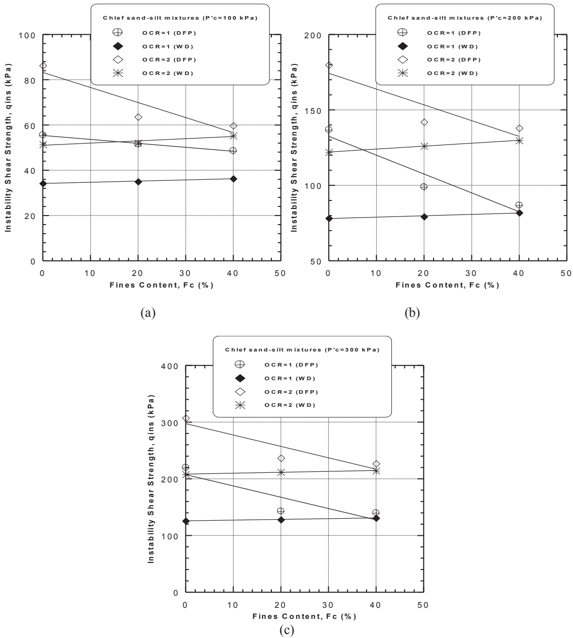
Figure 20: Instability shear strength of sand–silt mixtures versus fines content ( D_r = 52\% ): (a) P'_c = 100 kPa; (b) P'_c = 200 kPa; (c) P'_c = 300 kPa.
