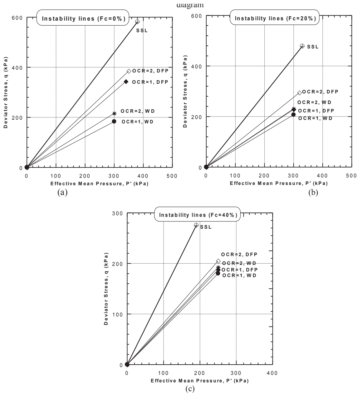
Figure 15: Instability and steady-state lines of Chlef sand-silt mixtures ( D_r = 52\% ): (a) F_c = 0\% , (b) F_c = 20\% and (c) F_c = 40\% .
