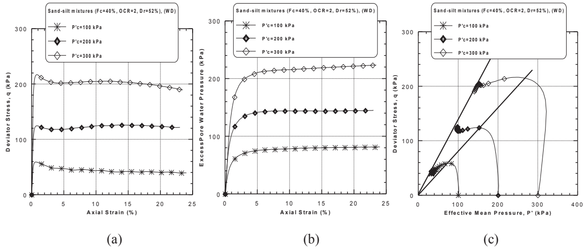
Figure 14: Undrained monotonic response of wet deposited sand-silt mixtures ( F_c = 40\% , OCR = 2 , D_r = 52\% ): (a) deviator stress versus axial strain, (b) excess pore water pressure versus axial strain and (c) stress path diagram.
