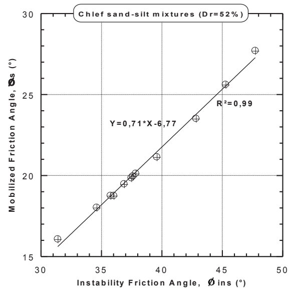
Figure 23: Mobilised friction angles versus instability friction angle of Chlef sand–silt mixtures.
