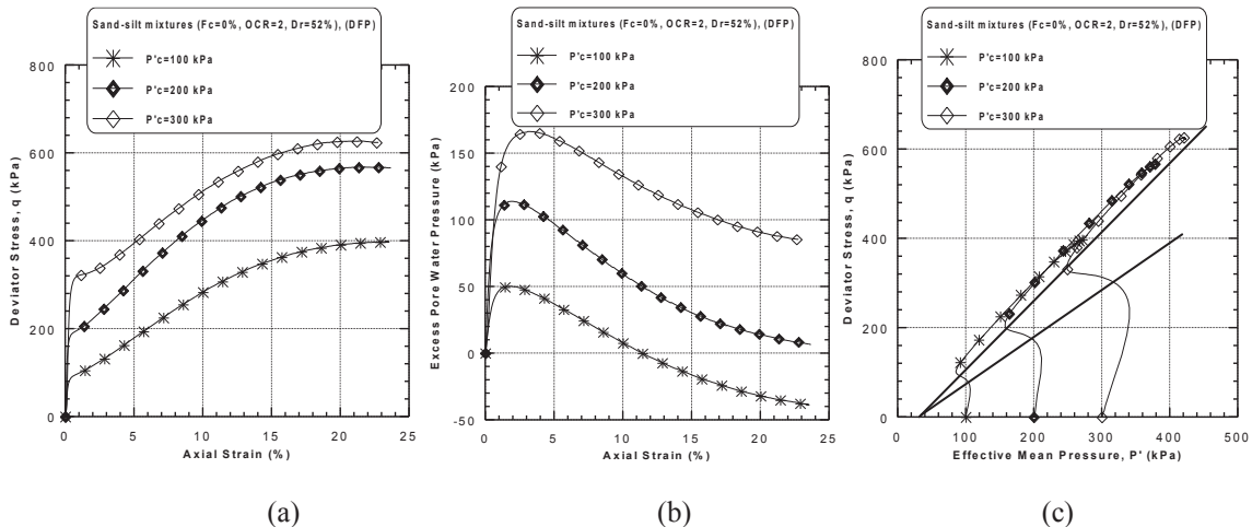
Figure 9: Undrained monotonic response of dry funnel pluviated sand-silt mixtures ( F_c = 0\% , OCR = 2 , D_r = 52\% ): (a) deviator stress versus axial strain, (b) excess pore water pressure versus axial strain and (c) stress path diagram.
