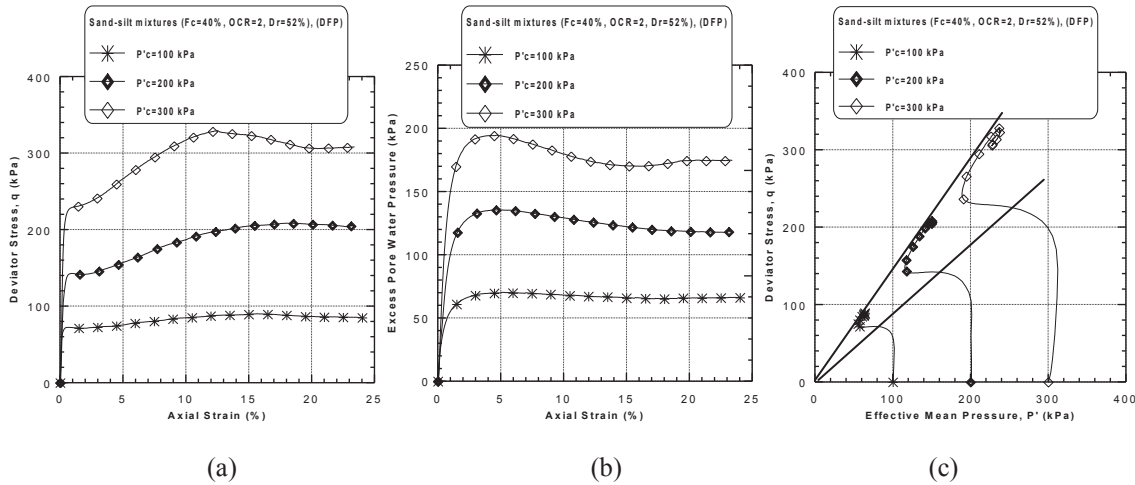
Figure 10: Undrained monotonic response of dry funnel pluviated sand–silt mixtures ( F_c = 40\% , OCR = 2 , D_r = 52\% ): (a) deviator stress versus axial strain, (b) excess pore water pressure versus axial strain and (c) stress path diagram.
