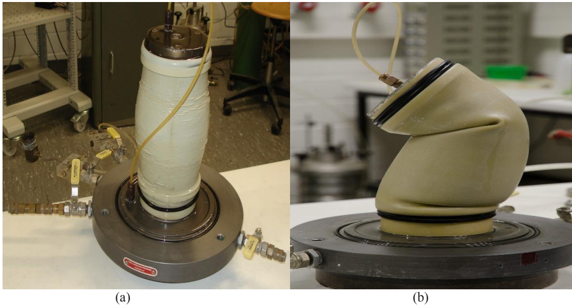
Figure 6: View of (a) dry funnel pluviated and (b) wet deposited samples after shearing.
