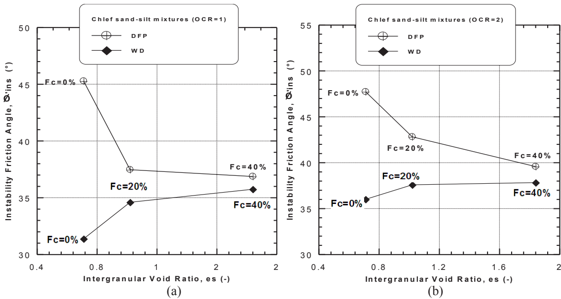
Figure 25: Instability friction angles versus intergranular void ratio: (a) OCR = 1 and (b) OCR = 2.
