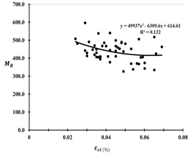
Figure 18: Relationship between M_R and crack initiation strain ( \epsilon_{ci} ).
