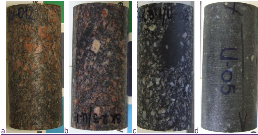
Figure 3: Main types of rock samples. (a, b) Megacryst-bearing, medium-grained, biotite monzogranites. (c) Medium-grained, biotite monzogranites with elongated monzonitic enclaves. (d) Quartz monzonite.
