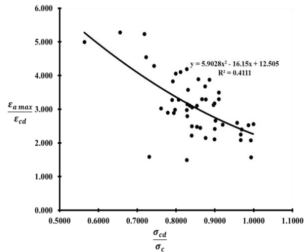
Figure 16: Relationship between \frac{\sigma_{cd}}{\sigma_c} and \frac{\epsilon_{a,max}}{\epsilon_{cd}} .
