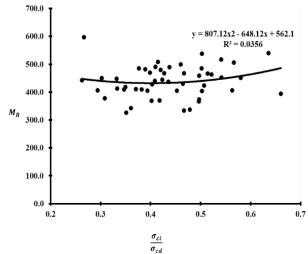
Figure 19: Relationship between M_R and \frac{\sigma_{ci}}{\sigma_{cd}} .
