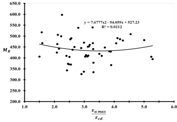
Figure 15: Relationship between M_R and \frac{\epsilon_{a,max}}{\epsilon_{cd}} .
