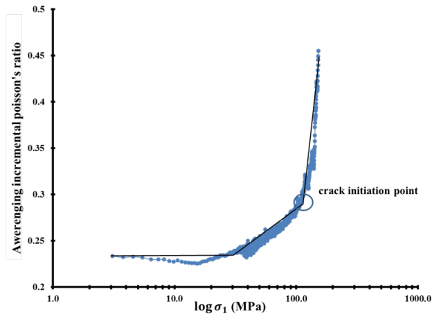
Figure 7: Poisson's ratio method for crack initiation threshold determination for Hungarian granitic rock sample (uniaxial compression case).
