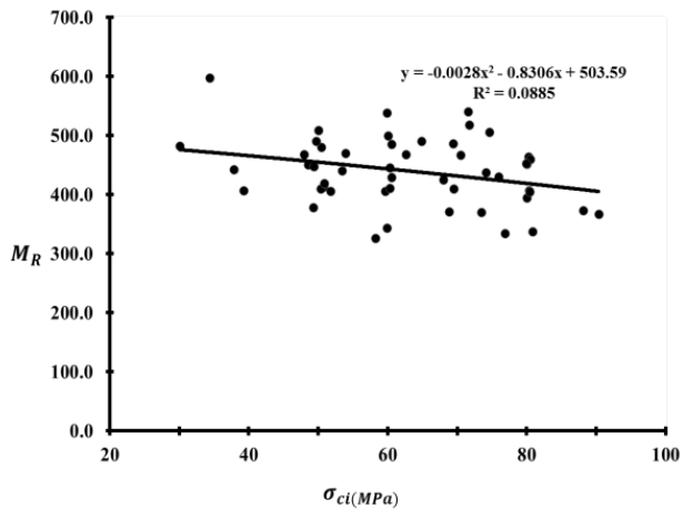
Figure 17: Relationship between M_R and crack initiation stress ( \sigma_{ci} ).
