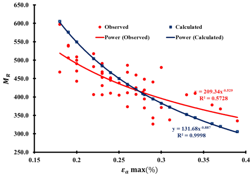
Figure 10: Observed and analytical (Eq. 1) relationship between \varepsilon_{a, \max} and M_R .
