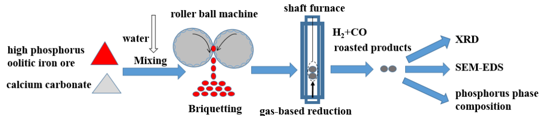
Fig. 2. Experimental procedures for the gas-based reduction process of a high phosphorus oolitic iron ore
