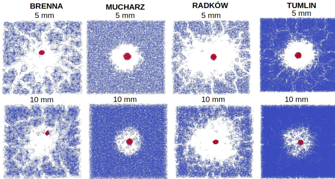
Figure 17: Network of fractures which appeared in the sample after impact resistance test. View of bonds.
