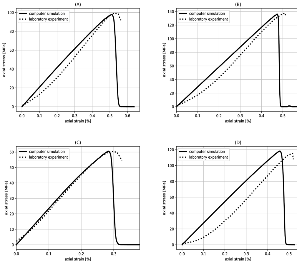
Figure 8: Comparison between numerical and laboratory stress-strain curves for selected samples: (A) Brenna BR2, (B) Mucharz MU1, (C) Radków RAD1 and (D) Tumlin TU2.
