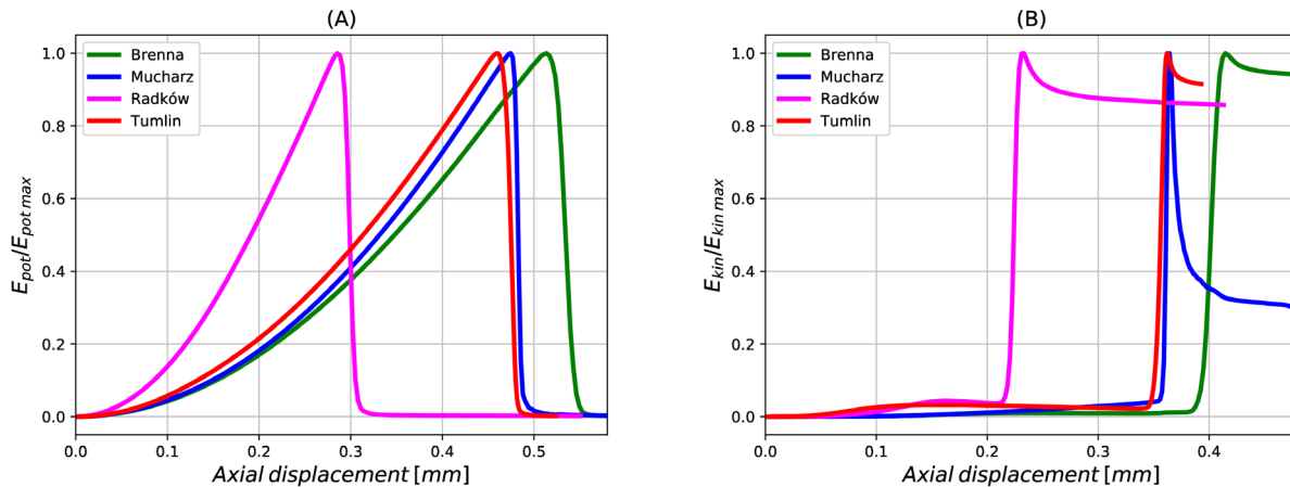
Figure 11: (A) Scaled potential energy of bonds E_{\text{pot}}/E_{\text{pot max}} and (B) scaled kinetic energy E_{\text{kin}}/E_{\text{kin max}} for all four types of sandstones.
