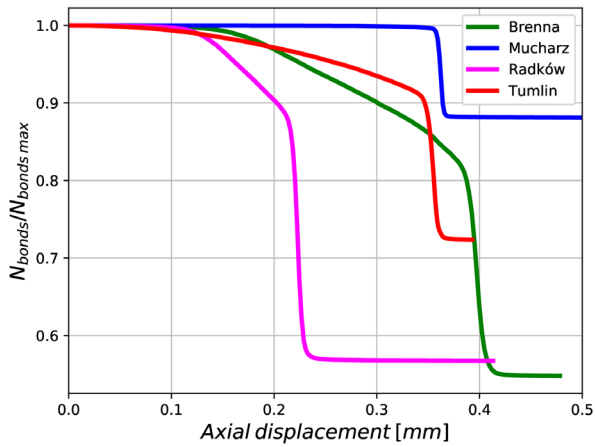
Figure 9: Scaled number of bonds N_{\text{bonds}}/N_{\text{bonds max}} (number of bonds divided by maximum number of bonds) inside the sample as a function of axial displacement for all four types of sandstones.
