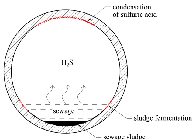
Figure 1: Concrete corrosion mechanism
