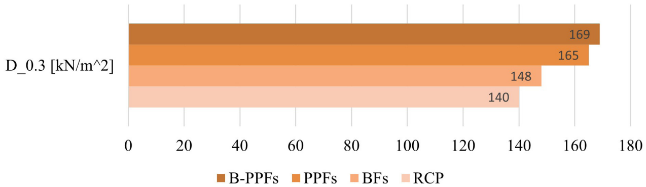
Figure 4: The service load of normalised pipe load-carrying capacity when the crack width is 0.3 mm for different reinforced concrete pipes (Deng et al. 2021a).
