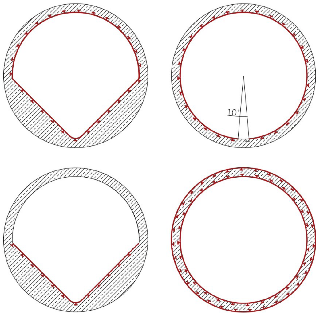
Figure 6: Different installation details of HDPE liners.
