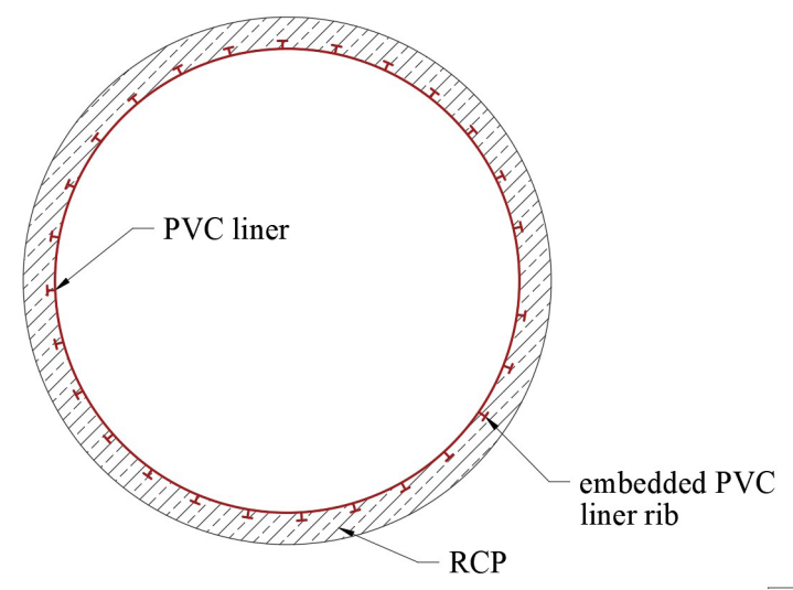
Figure 7: Reinforced concrete pipe with PVC liner
