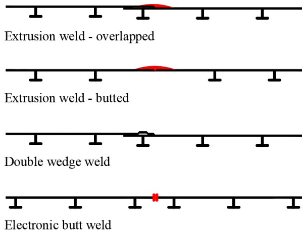
Figure 5: HDPE weld types.
