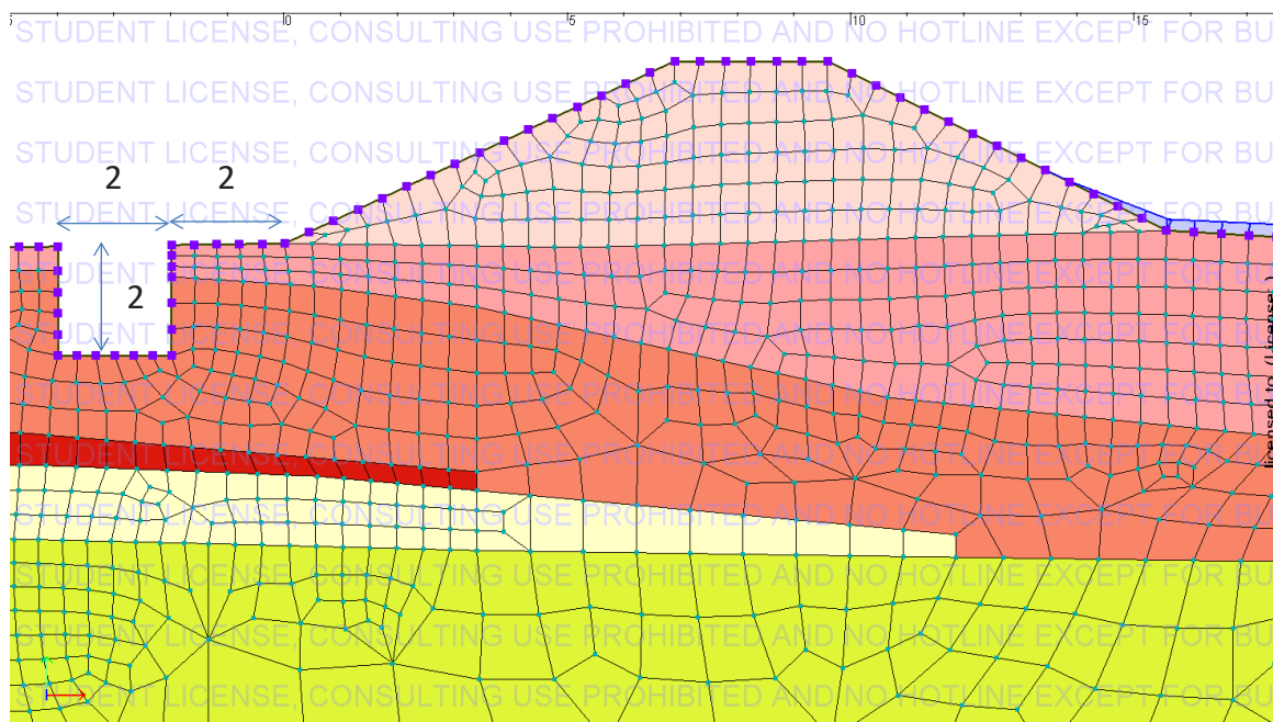
Figure 5: Numerical model of the embankment (a) with shallow excavation existing state and (b) with open excavation.
