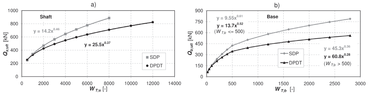
Figure 9: Derived relationships between pile load limit resistances Q_{s,ult} (a) and Q_{b,ult} (b) and representative screwing resistances W_{Ts} (a) and W_{Tb} (b) separately for SDP and DPDT drill augers.
