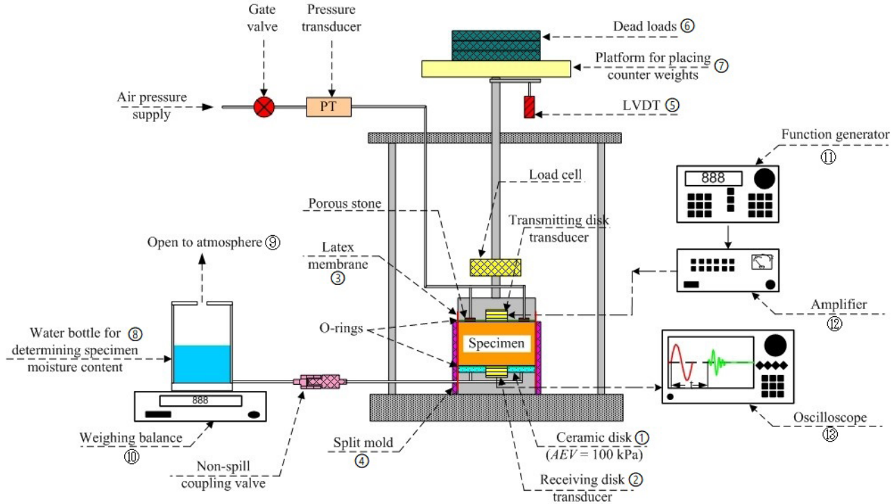
Figure 4: Schematic layout of modified SWCC wave velocity apparatus.
