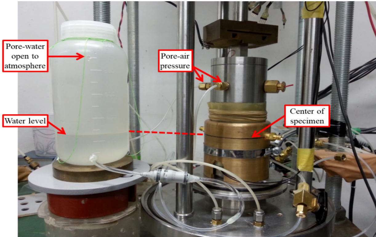
Figure 3: Water injection/drainage setup.
