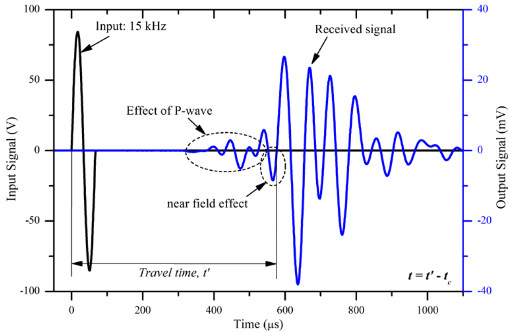
Figure 6: Travel time determination of shear wave signals.
