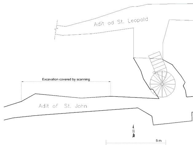
Figure 2: Location of the scanned 7.5-m fragment of the adit on the underground track “St. Johannes” Mine in Krobnica. In the vicinity of the measurement site, there is a shaft connecting both adits (St. Leopold below and St John above).
