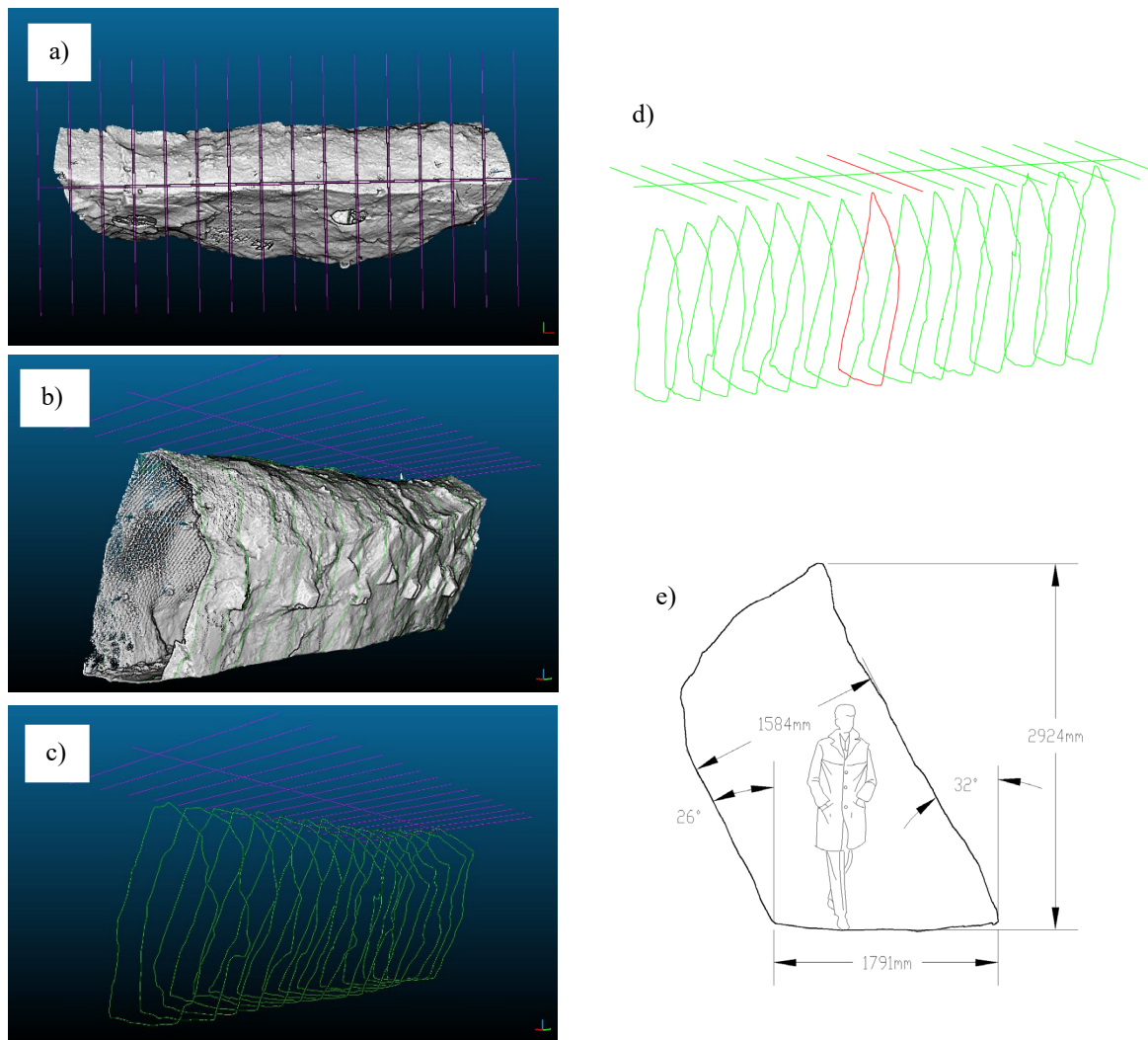
Figure 6: (a–c) Generating 2D cross sections from (a) “point cloud” in CloudCompare software and (d, e) dimensioning of a selected characteristic cross section.
