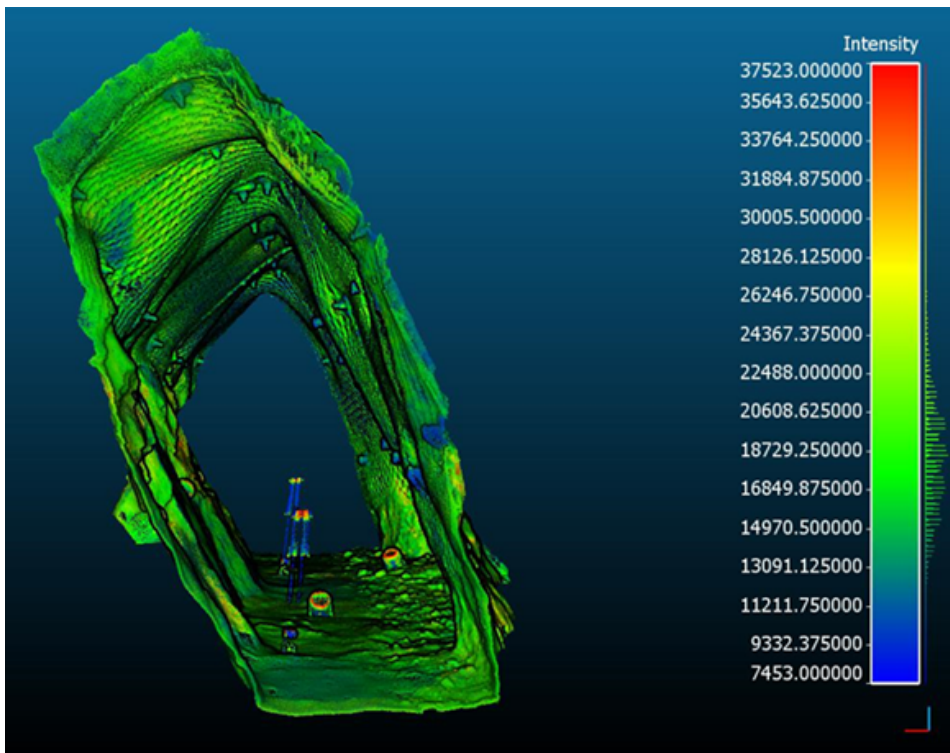
Figure 5: “Point cloud” visualization of a fragment of the St. John adit, displayed by the value of the reflection intensity parameter.
