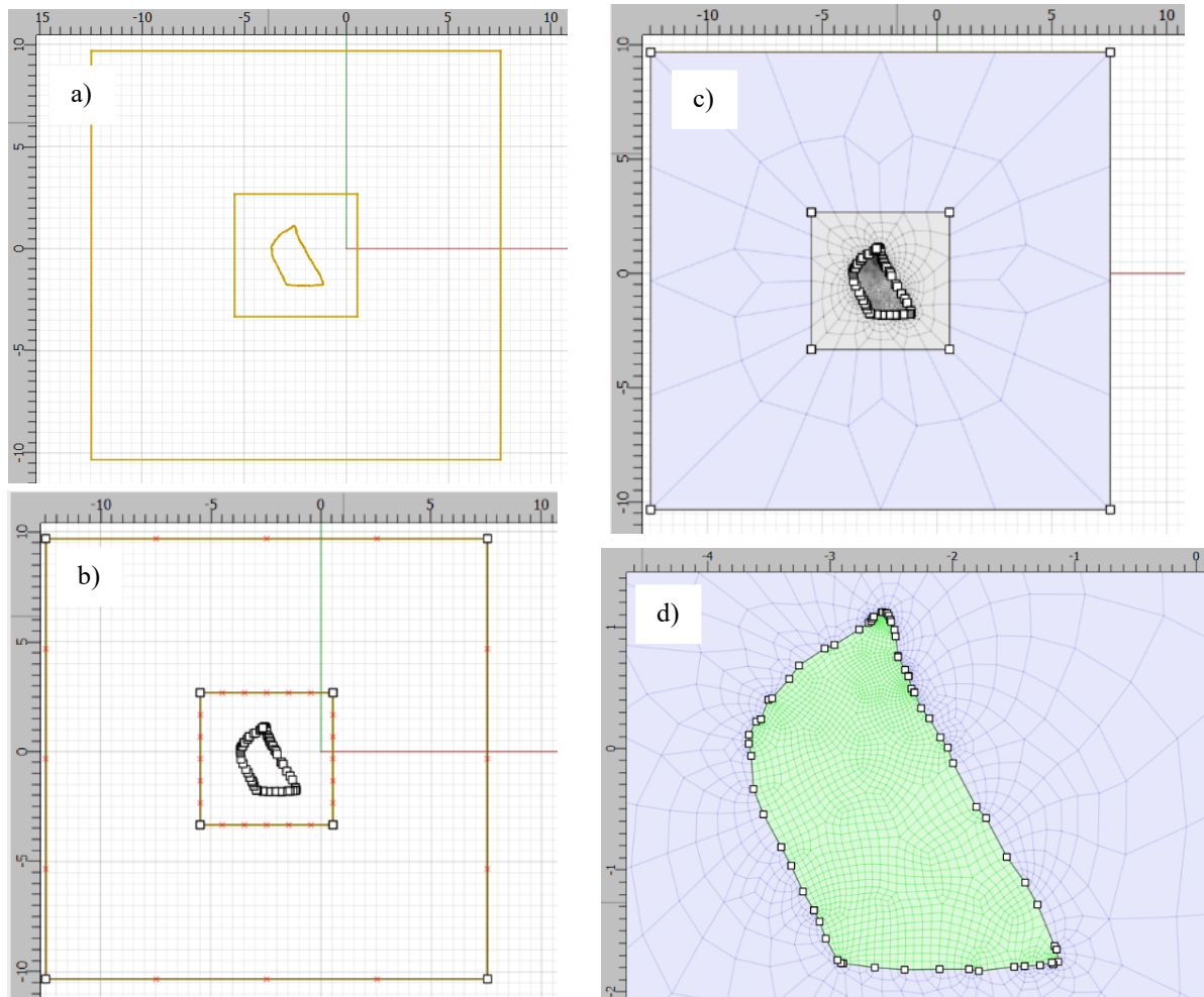
Figure 7: (a, b) Creating the cross sectional geometry of the scanned fragment of the adit and (c, d) its discretization in FLAC 3D Itasca v.9.0 software, sketch option.
