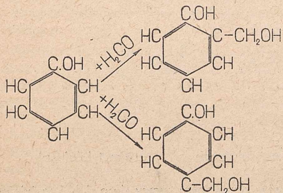
o-metylofenol
