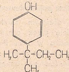
amylofenol
