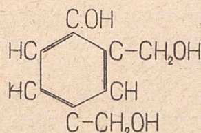
o, p-dwumetylolofenol
