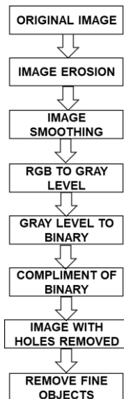
Fig. 2. Flow chart of edge detection process
