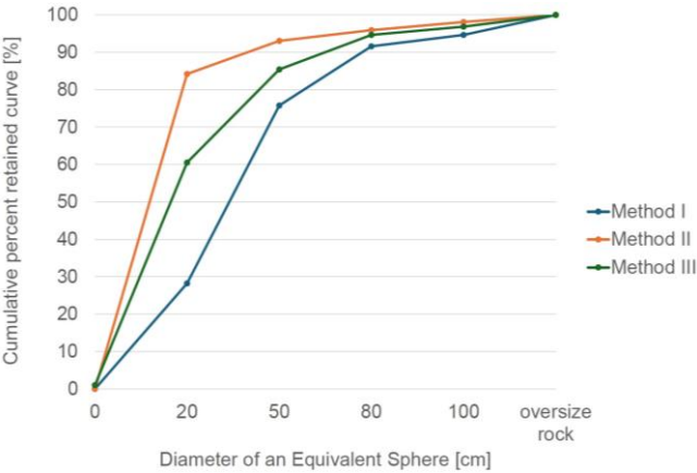
Fig. 9. Grain size distribution curves of the representative fragment of the muck pile obtained using Method I, Method II and Method III
