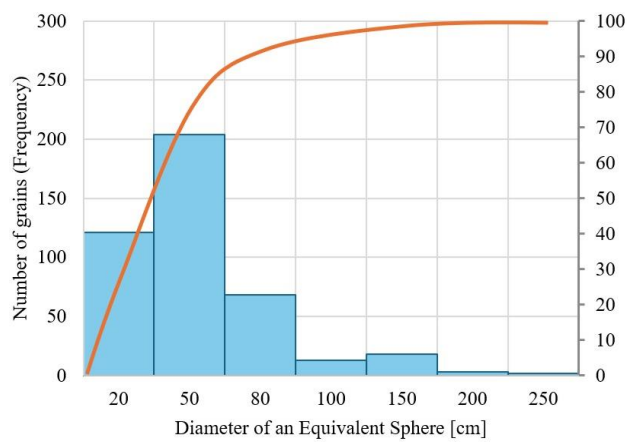
Fig. 3. Grain size distribution curve prepared using the manual method
