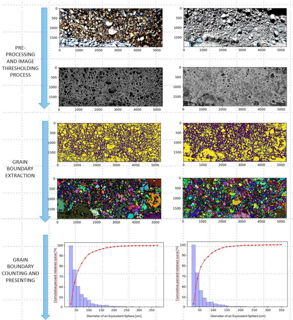
Fig. 7. Individual outputs of the grain size distribution curve generation procedure using open-source algorithm in Matlab
