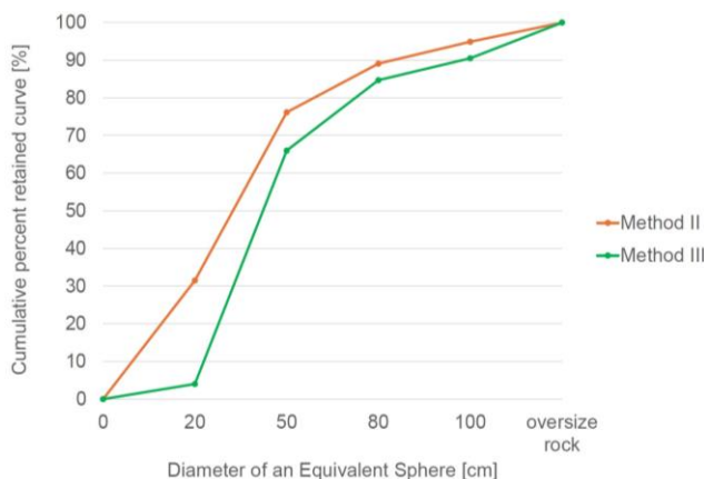
Fig. 10. Grain size distribution curves of the representative fragment of the muck pile obtained using Method II and Method III
