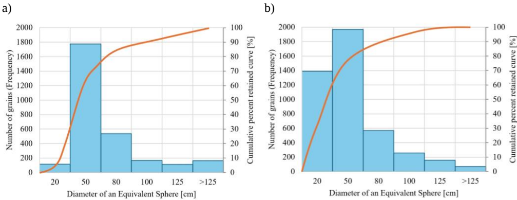
Fig. 8. The result of the grain size distribution of the entire muck pile (a) and a representative fragment of the muck pile (b) obtained using open-source algorithm in Matlab
