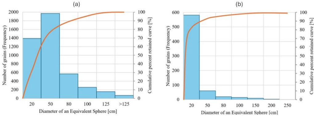
Fig. 5. Grain size distribution of the entire muck pile (a) and a representative fragment of the muck pile (b) generated in Wipfrag Deep Learning mode
