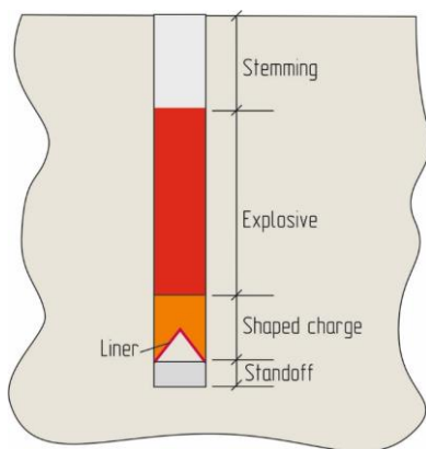
Fig. 4. Construction of an additional borehole
