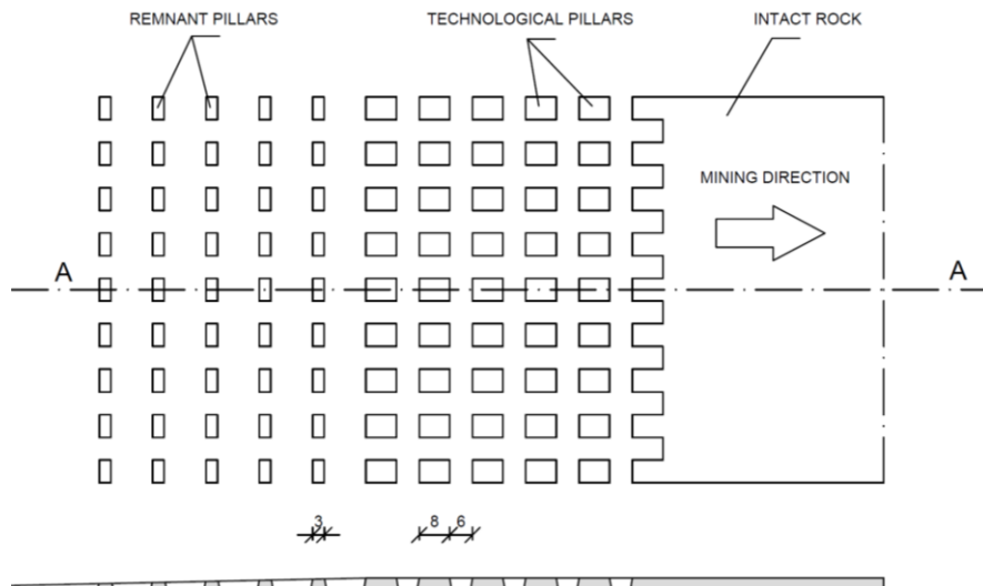
Fig. 2. Room and pillar mining system with roof deflection
