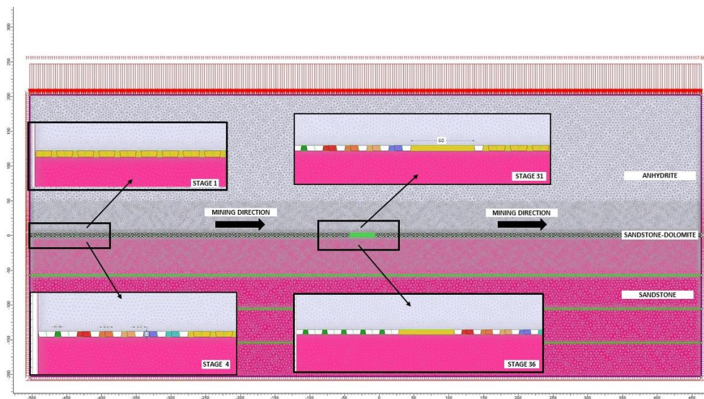
Fig. 4. Numerical model for the remnant width 60 m
