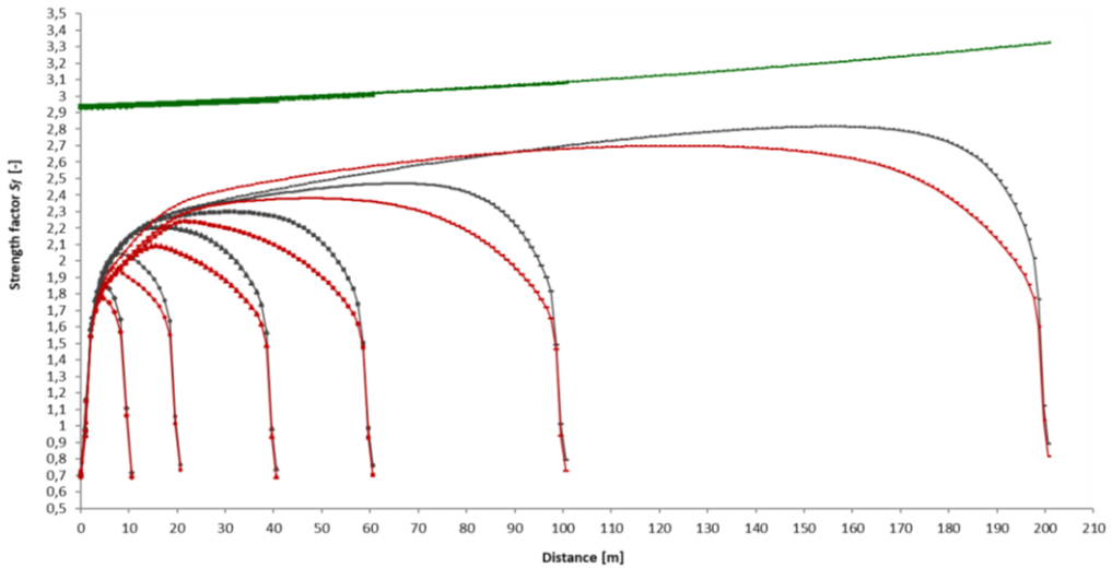
Fig. 9. Comparison between strength factor S_f inside the remnant of different size: 10, 20, 40, 60, 100, and 200 m
