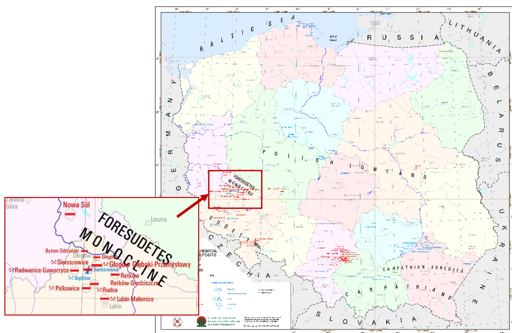
Fig. 1. Location of the copper deposit and mines in Poland (based on: Polish Geological Institute, 2024)
