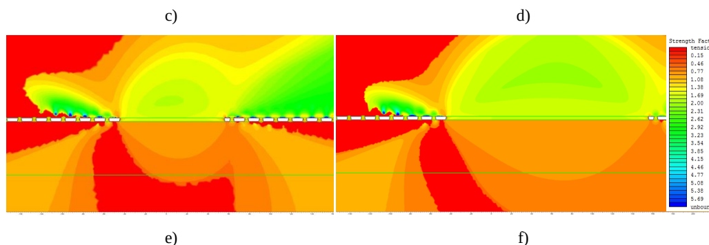
Fig. 7. Distribution of strength factor S_f for the front distance approximately 400 m from the remnant edge – 59th calculation step for different remnant width:
