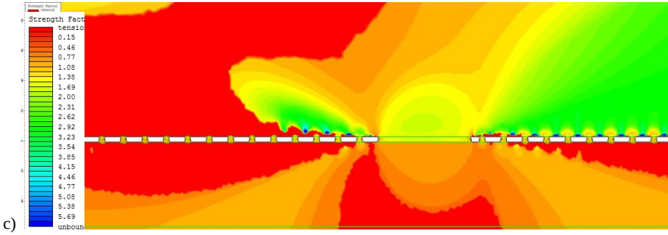
Fig. 6. Distribution of strength factor S_f for the front distance approximately: a) 300 m – 19th calculation step, b) 620 m (100 m from the remnant edge) – 38th calculation step, c) 920 m (400 m from the remnant edge) – 59th calculation step
