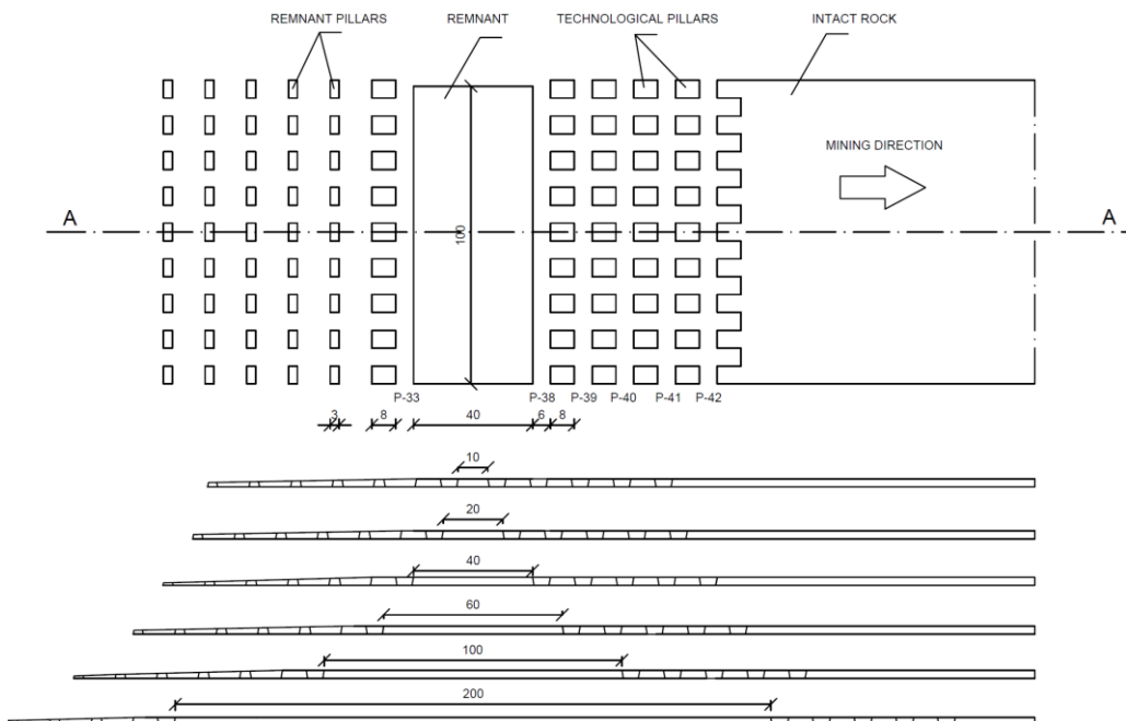
Fig. 3. Mining field where the room and pillar mining system with roof deflection is used and 6 variants of remnant width: 10, 20, 40, 60, 100, and 200 m are left behind
