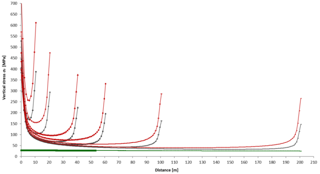
Fig. 8. Comparison between vertical stresses \sigma_y inside the remnant of different size: 10, 20, 40, 60, 100, and 200 m
