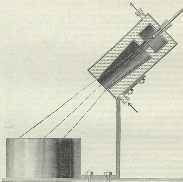
Pyrometer for various intensities.
