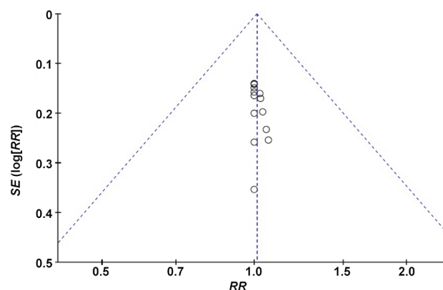
Fig. 3. Funnel plot displaying the heterogeneity between the studies included in the meta-analysis
