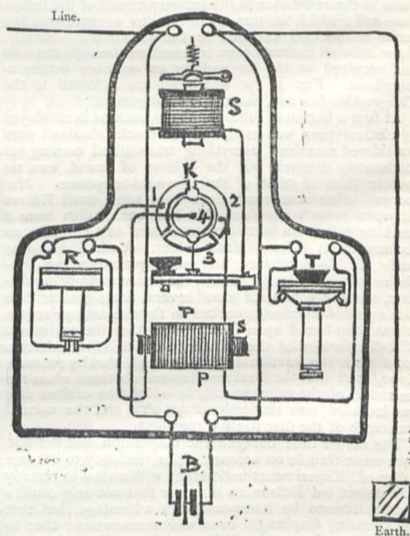
FIG. 3.—Electric arrangement of the Carbon Telephone.
