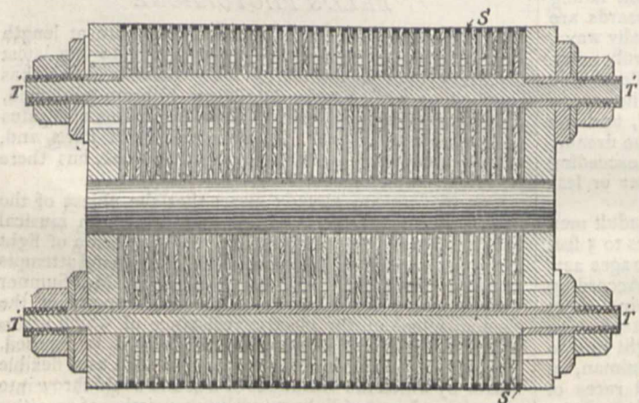
FIG. 3.—Section of the Selenium Receiver, shown as S in Fig. 2.
