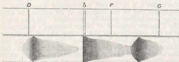
No. 1.—Spectrum of Crul's Comet, October 15 and 16.
