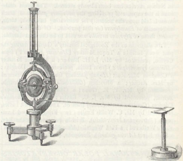
FIG. 27.—Gyroscope; general view.
