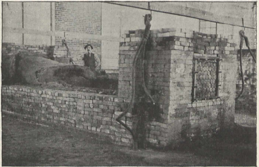
FIG. 2.—Furnace opened to show formation of carborundum around the core.
