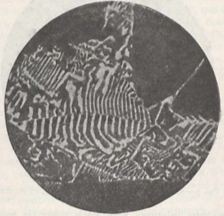
FIG. 1.—Alloy of silver, 66 per cent.; antimony, 34 per cent.
