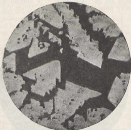
FIG. 3.—Alloy of tin, 75 per cent. ; antimony, 25 per cent.
