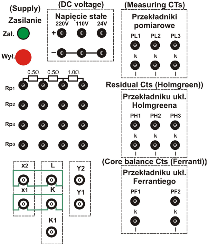
Fig.2.2. View of the face panel for setting and connections
