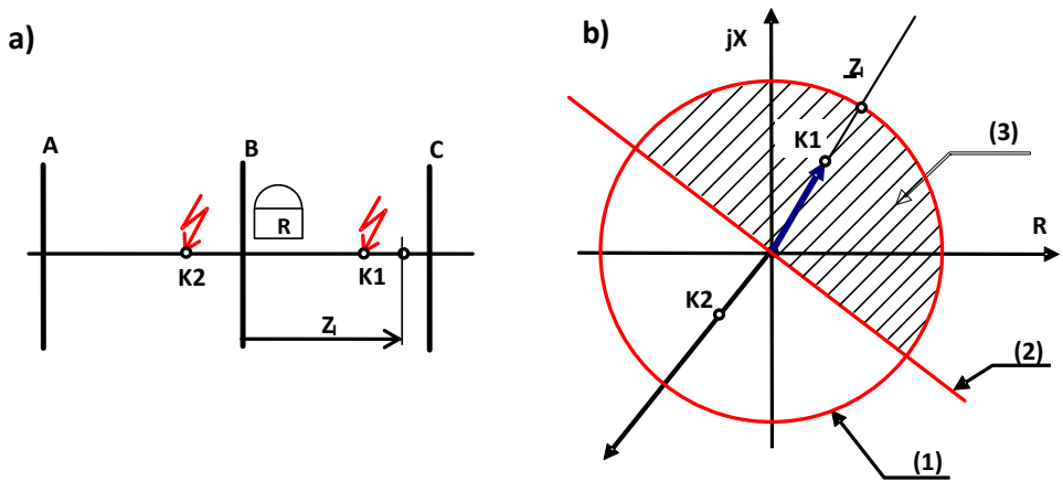
Fig.1.6. Explanation of role of a directional-sensing unit; a) scheme of line being protected (R – distance relay to protect BC line distance, K1,K2 – fault locations), b) operational threshold characteristic (1 – plain impedance characteristic, 2 – directional characteristic, 3 – zone of operation)
