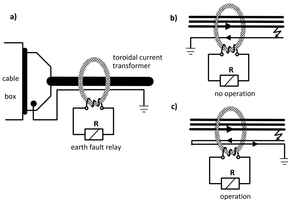
Fig.1.6. Typical application of the core balance (Ferranti) current transformer for ground fault protection with metallic sheath conductors
