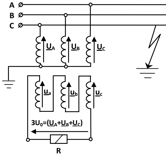
Fig.1.2. Connections of voltage transformer to detect zero-sequence voltage component (a neutral voltage displacement)
