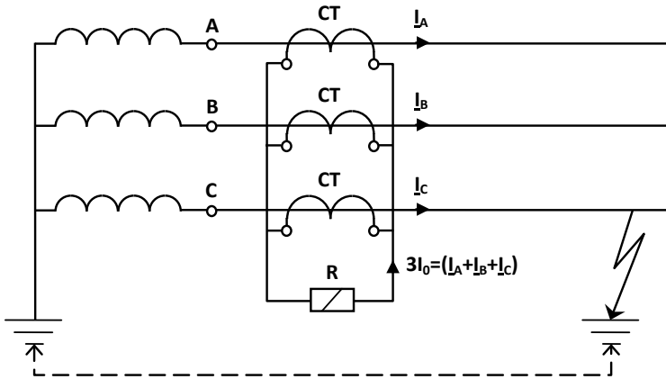
Fig.1.1. Principle of residual (Holmgreen) CT connection (CTs – line current transformers)
