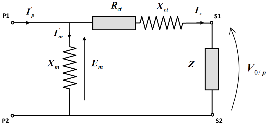
Fig. 1.2. Simplified equivalent scheme of current transformer
