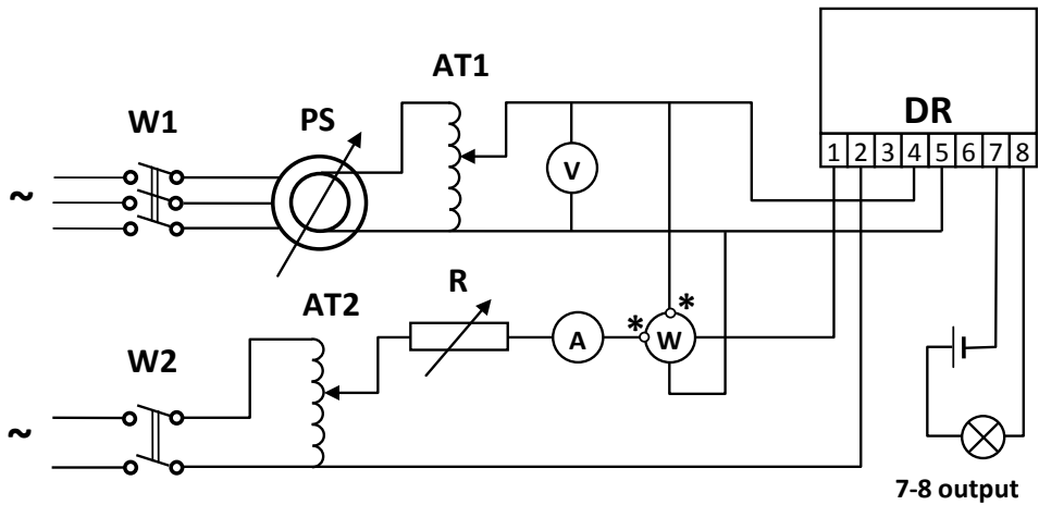
Fig.3.1. Typical circuit for the measurement of RCA; PS – phase shifter, AT1, AT2 – autotransformers, DR – directional relay
