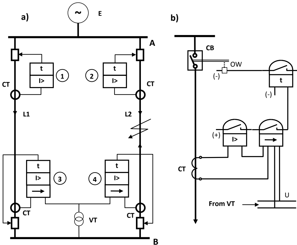
Fig.1.1. Example of application of directional relays; a) ring type distribution system with directional overcurrent protections, b) schematic diagram of time delayed overcurrent protection
