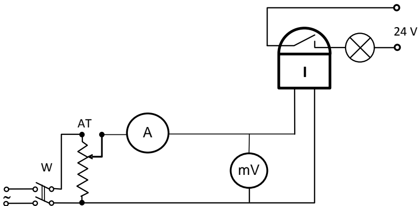
Fig .5.2. Typical circuit for testing instantaneous overcurrent relays
