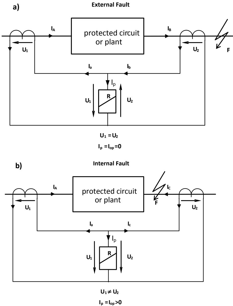
Fig.1.1. Basic current differential scheme illustrated for the protection of a zone with two circuits: a) normal state or/and external fault, b) internal fault
