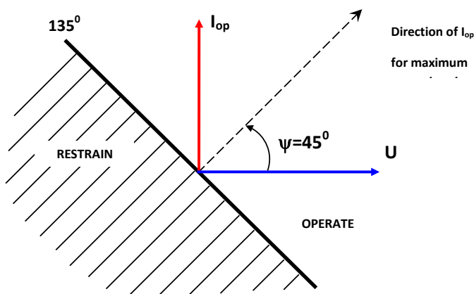
Fig.2.3. Example of directional relay characteristic
