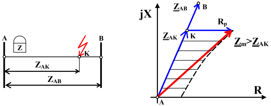
Fig.1.4. Variation of the measured impedance Z_m due to ground fault resistance R_p
