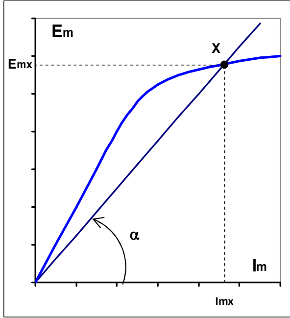
Fig.1.5. Illustration for the ALF determination
