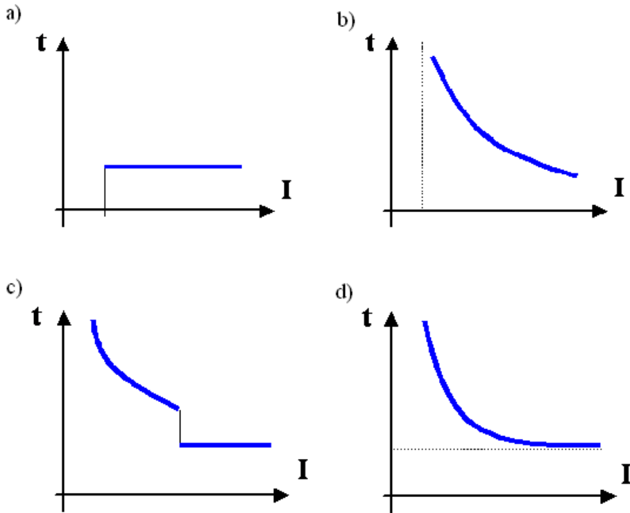
Fig.2.1. Time – current characteristics of over-current relays; a) definite time, b) inverse time, c) inverse time with short-circuit pickup, d) inverse definite minimum time
