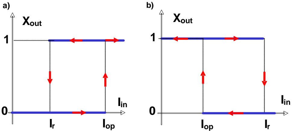
Fig.1.2. Illustration of over-current (a) and undercurrent (b) relay operation ( X_{out} – output signal, I_{in} – input current, I_{op} , I_r – operation and release value respectively)
