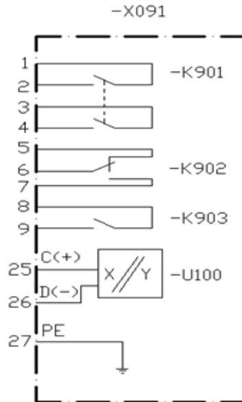
Fig.2.4. Schematic diagram of the MiCOM P631 relay (internal wiring diagram of module contacts)
