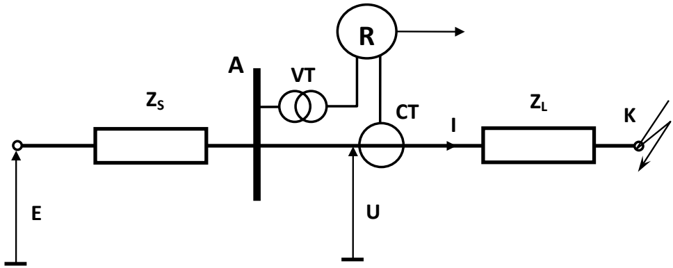
Fig.2.8. Explanation of operation conditions of directional relay under short circuit in feeder; A – source substation, Z_s – source impedance (behind relay location), Z_L – line impedance (in front of relay location), VT, CT – voltage and current transformers respectively, I, U – short circuit current and voltage (residual)
