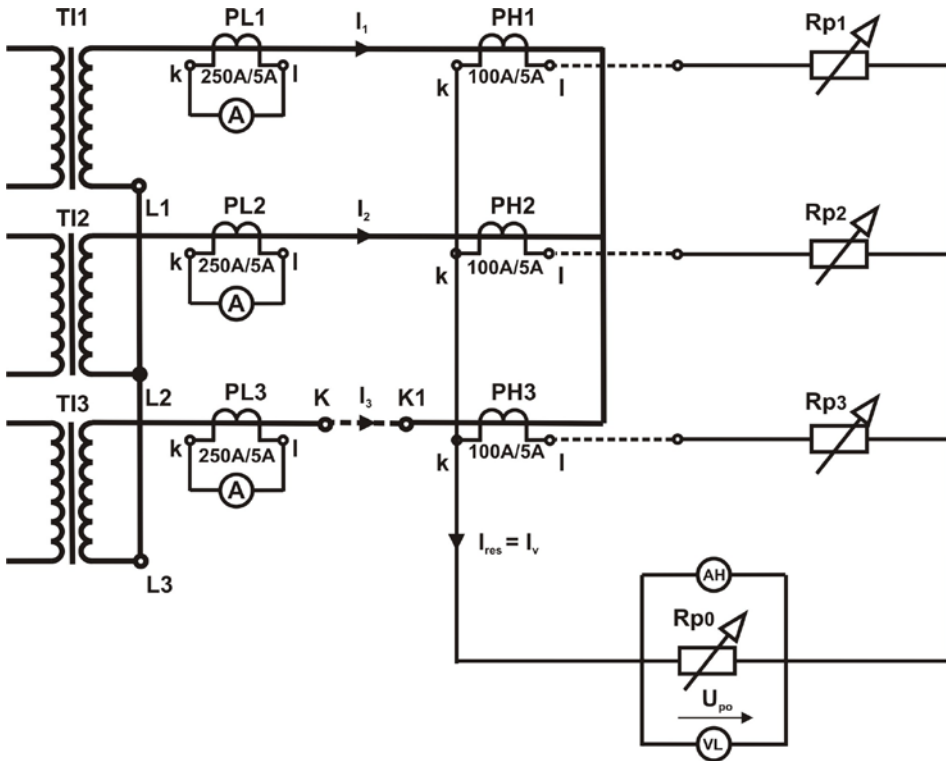
Fig.2.1 Diagram of electric circuit for errors current measurement of the residual CTs connection; TI1...TI3 – supplying transformers, PL1...PL3 – measuring current transformers, PH1...PH3 – line transformers of the Holmgreen system, AH – harmonics analyzer, VL – electronic voltmeter.
