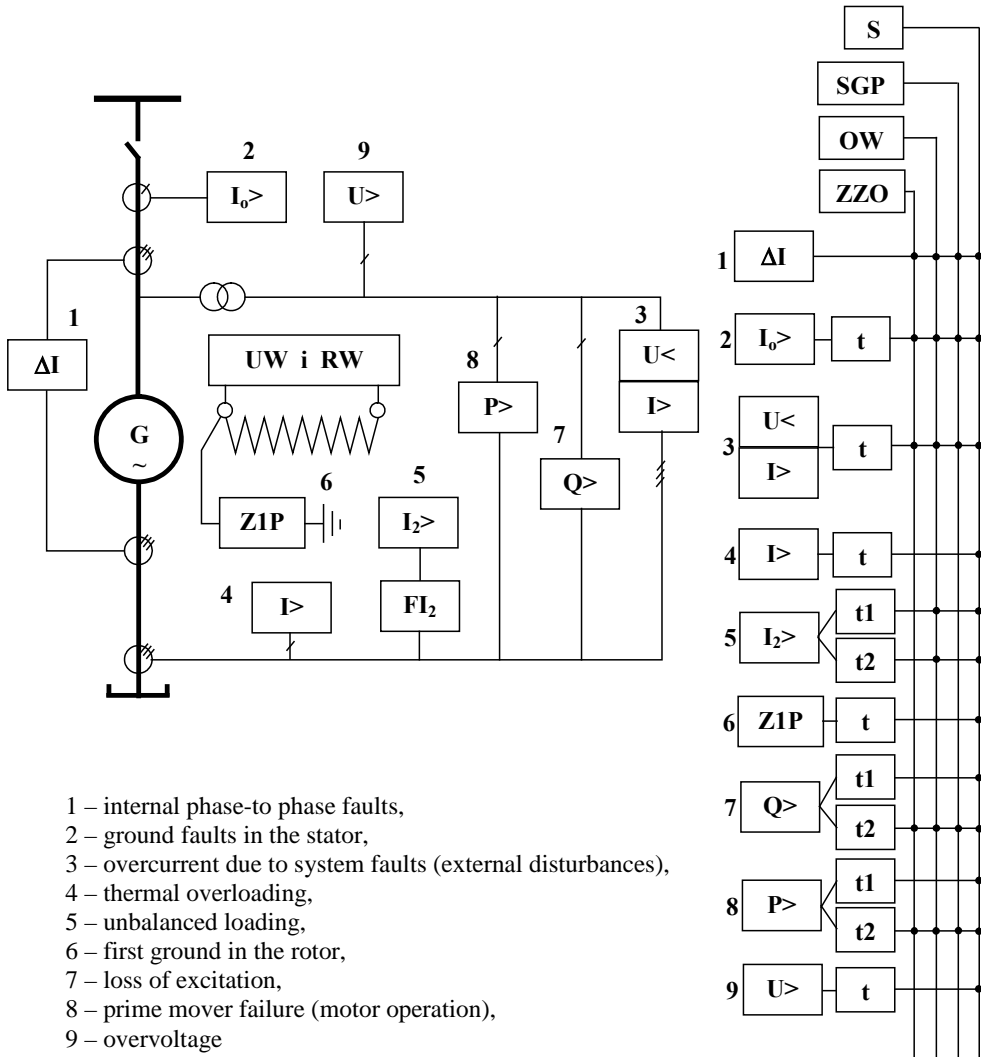
Fig.2.1. Schematic of the protection for the synchronous generator model
