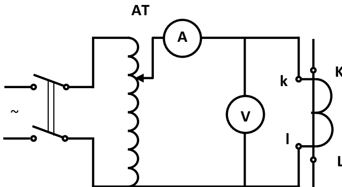
Fig.2.3. Typical circuit for the measurement of CTs magnetization characteristic
