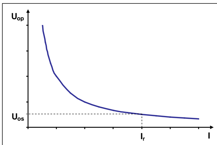
Fig.2.5. Operating characteristic U_{op}=f(I) of directional relay
