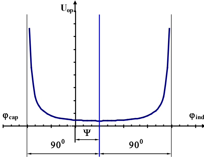
Fig.2.6. Angular characteristic of directional relay
