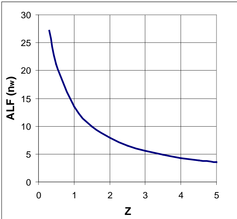
Fig.1.4. ALF value versus output burden ( Z ) of the CT
