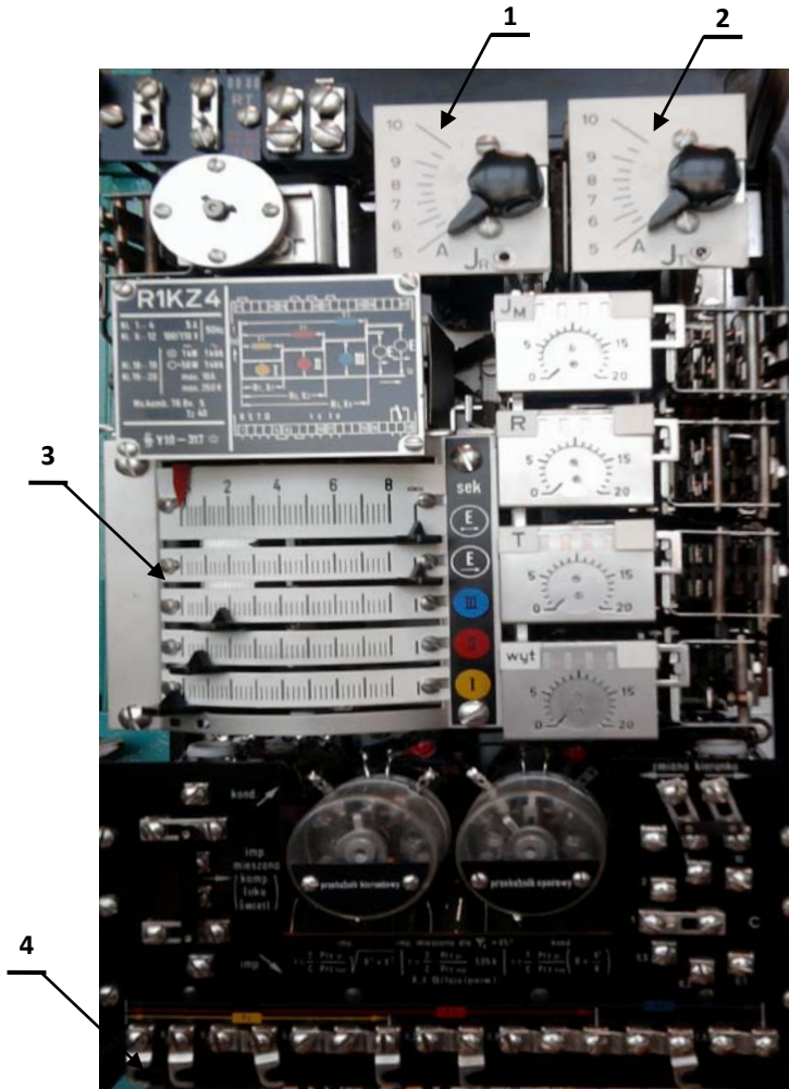
Fig.2.1. General view of the R1KZ4 type relay (Siemens); 1, 2 - over-current threshold sensing units I_R and I_T , 3 - scale for timing unit, 4 - shunting clamps
