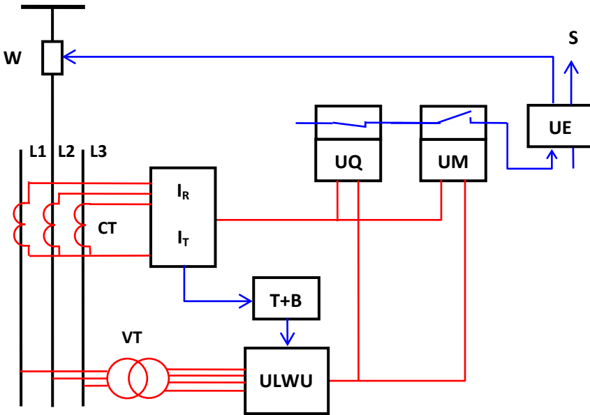
Fig.2.2. Functional block diagram of the R1KZ4 relay; I_R , I_T – over-current sensing units, UM – measuring unit, UQ – directional-sensing element, T+B – timing and setting unit, ULWU – logical function-selection element, UE – output and tripping block.
