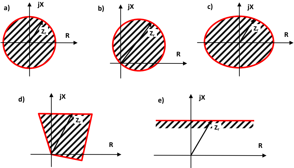
Fig.1.5. Selected distance characteristics: a) plain impedance, b) mho, c) elliptical, d) quadrilateral, e) reactance
