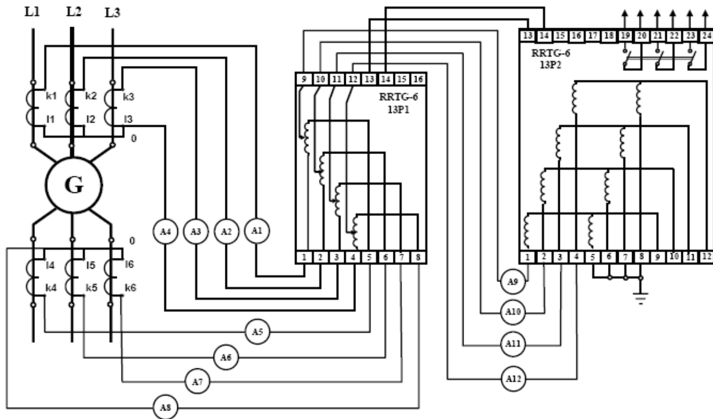
Fig. 4.1. Circuit diagram of the differential protection of RRTG-6 type of the generator
