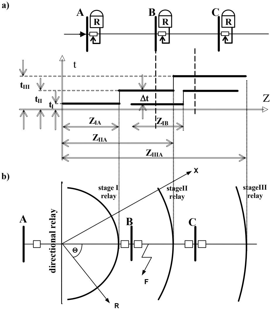
Fig.1.1. Distance protection utilizing plain impedance relays; a) time-impedance characteristics, b) plain impedance characteristics, Z_I - Z_{III} – impedance stages range, \Delta t – time lag,
