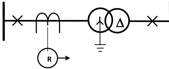
Fig.2.4. Setting of directional relays for selected application
