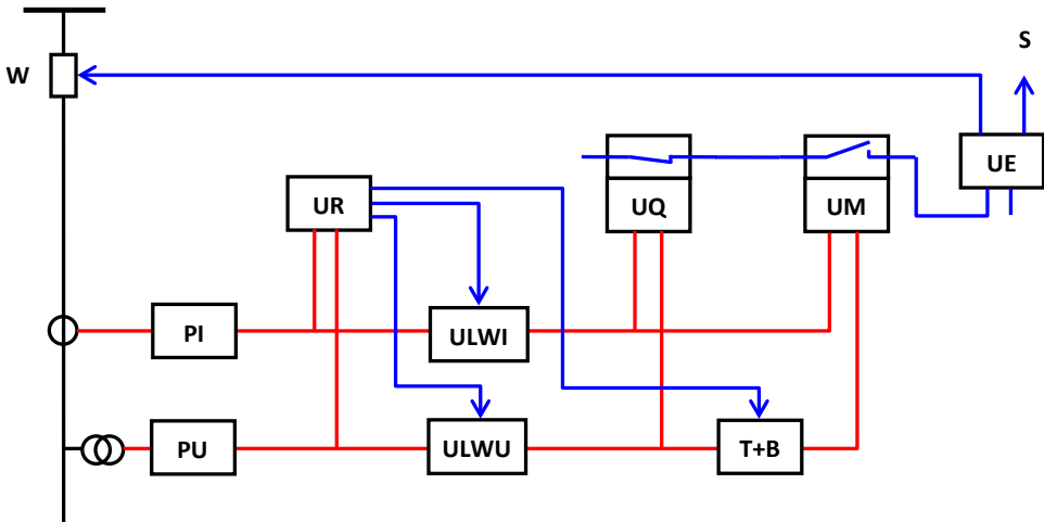
Fig.1.2. Block diagram of one measurement system distance relay; PI, PU – current and voltage convertors, UR – operational unit (over-current or under-impedance), ULWI, ULWU – logical function-selection elements, T+B – time setting unit (voltage and impedance zone), UQ = directional-sensing-element, UM – measuring unit, UE – output and tripping block
