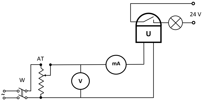
Fig.5.1. Typical circuit for testing instantaneous over- and/or -under-voltage relays
