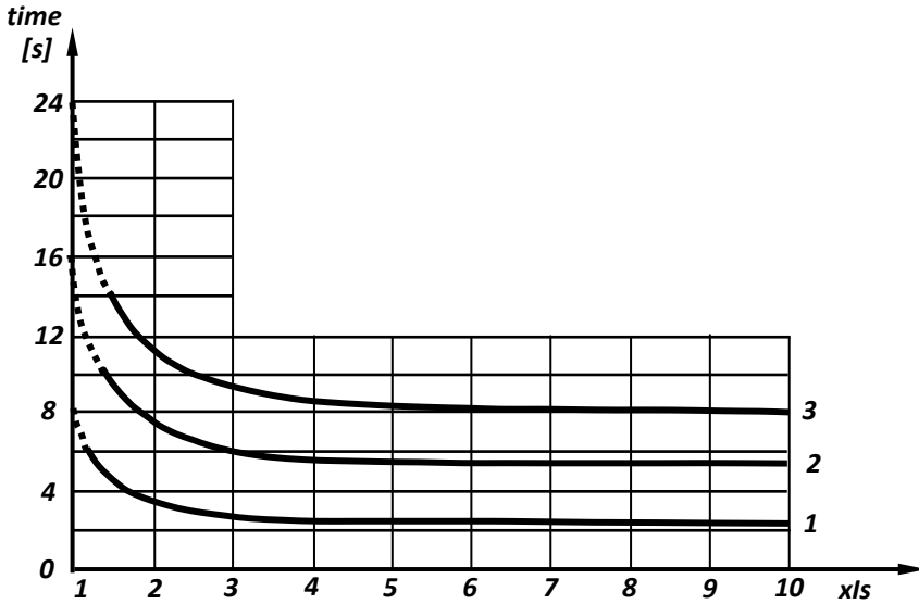
Fig.2.5. Time – current characteristics of RIz-104 relay (1- for t_n=8s , 2 – t_n=16s , 3- t_n=24s )
