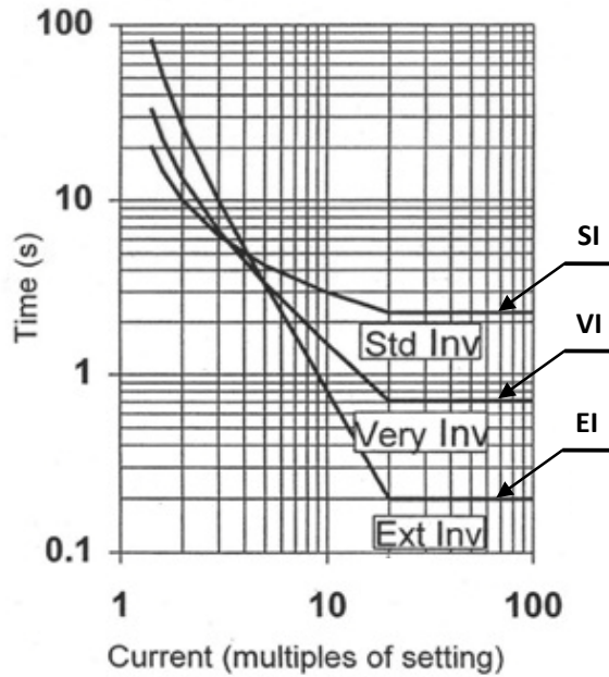
Fig.2.3. IDMT characteristics defined by IEC 255-4 standard (Standard Inverse (SI) for cable circuits, Very Inverse (VI) for overhead line circuits, Extremely Inverse (EI) for transformers)
