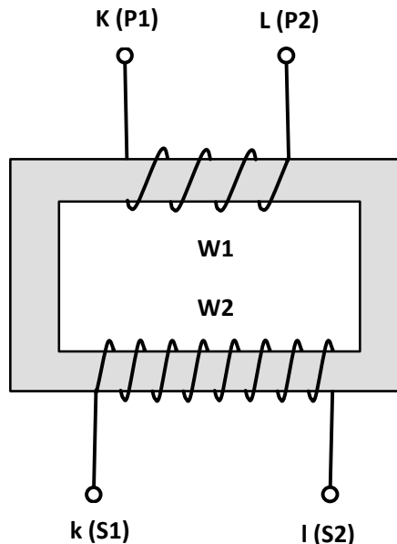
Fig. 1.1. Schematic diagram of a current transformer
