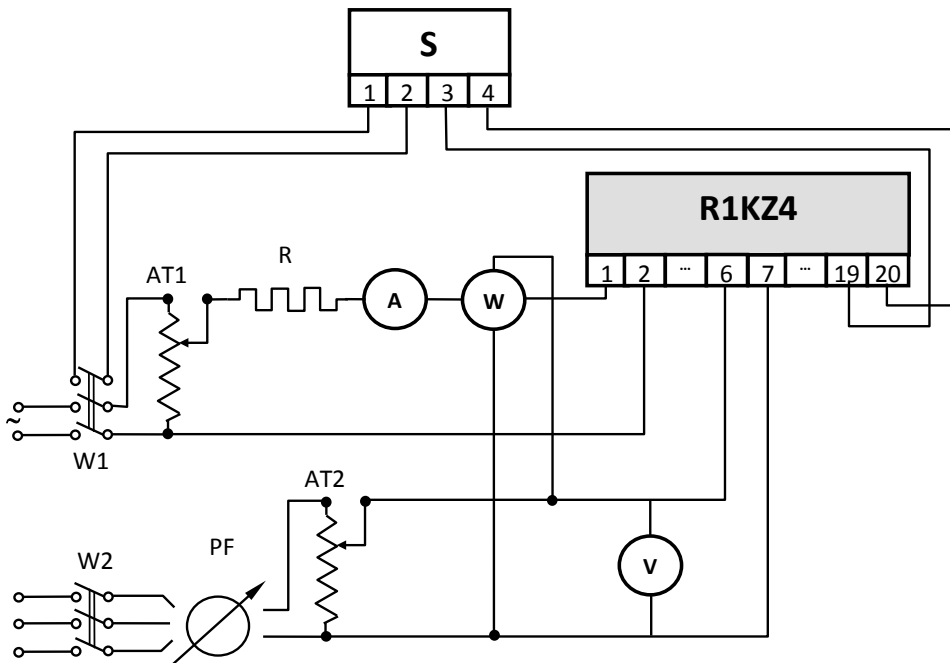
Fig.2.3. Schematic diagram of measuring circuit for testing R1KZ4 relay( A – ammeter, V – voltmeter, W – wattmeter, W1, W2 – switches, S – stop watch, AT1, AT2 – autotransformers, PF – phase shifter
