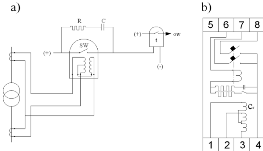
Fig.2.3. Schematic diagram of the TG-3 relay (a), SW – vibrating contact, R, C – elements of contact protection circuit, b) internal connection
