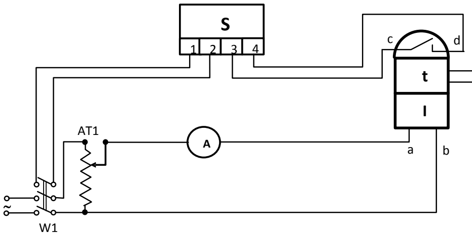
Fig.3.1. Typical circuit for the measurement of operational characteristics
