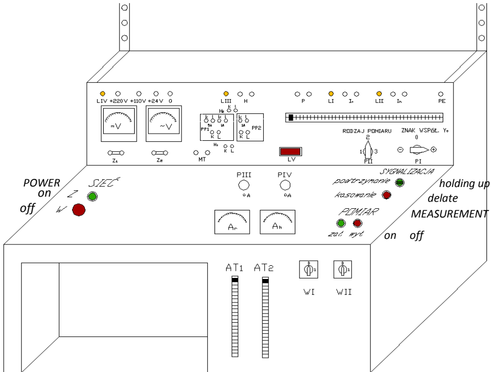
Fig.2.1. General view of laboratory stand for testing differential relays
