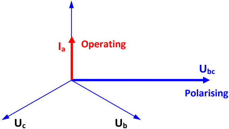
Fig.2.1. Illustration of choice of voltage reference
