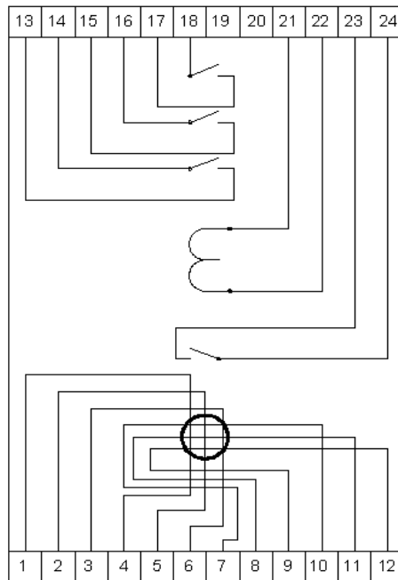
Fig.2.2. Internal connection of RQS-2 relay
