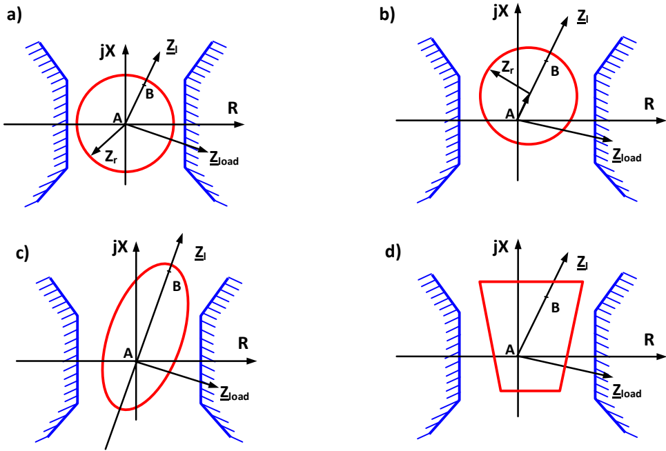
Fig.1.3. Distance relay characteristics on the R-X diagram; Z_r – characteristic impedance, Z_i – short-circuit impedance, a) for lines below 100km, b) for lines of around 100km, c) d) – lines over 100km
