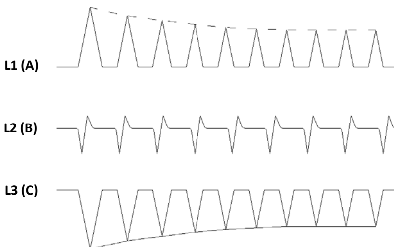
Fig.1.3. Illustration of magnetizing inrush current when switching on transformer under out of load operation
