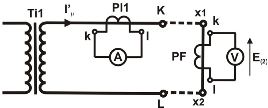
Fig.2.3. Circuit for derivation of voltage-current, magnetizing characteristic of the Ferranti CT (PF – core balance CT, PL1 – measuring CT)
