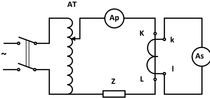
Fig.2.2. Circuit for the measurement of transformation ratio
