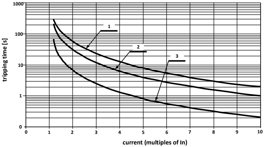
Fig. 2.7. Selected time – current characteristics for various initial thermal state \Theta (1 - \Theta=0 ; 2 - \Theta=0.5 ; 3 - \Theta=0.9 ; I_n – rated current)
