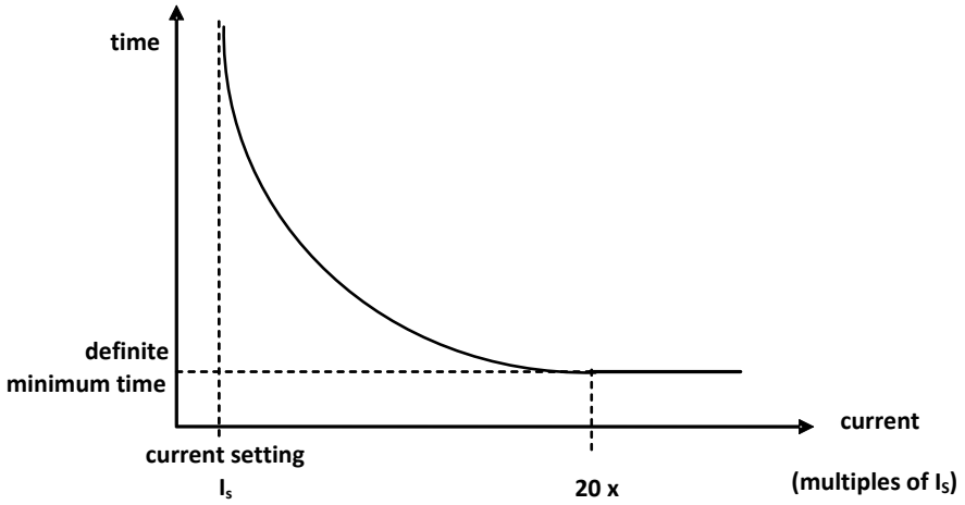
Fig.2.2. Inverse definite minimum time (IDMT) characteristic
