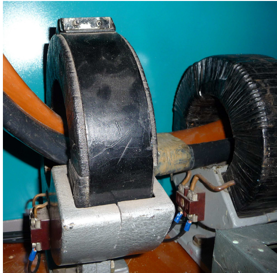
Fig.1.5. Lab model of Ferranti CTs
