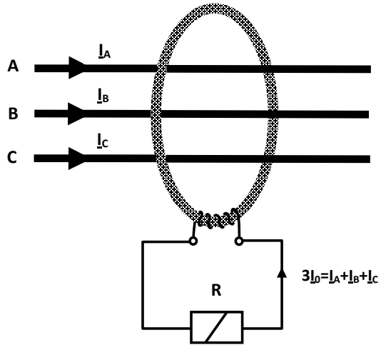
Fig.1.4. Idea of the core balance current transformer (R – ground fault relay)
