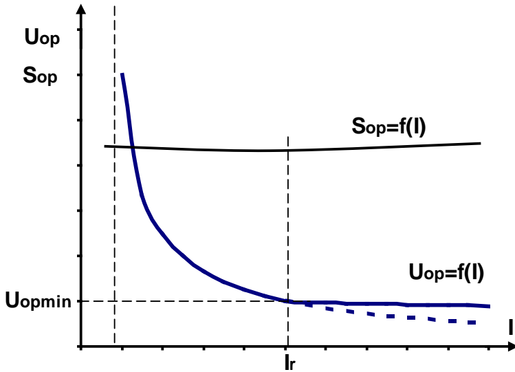
Fig.3.2. Characteristic U_{op}=f(I) and S_{op}=f(I) for electromechanical directional relay as an example
