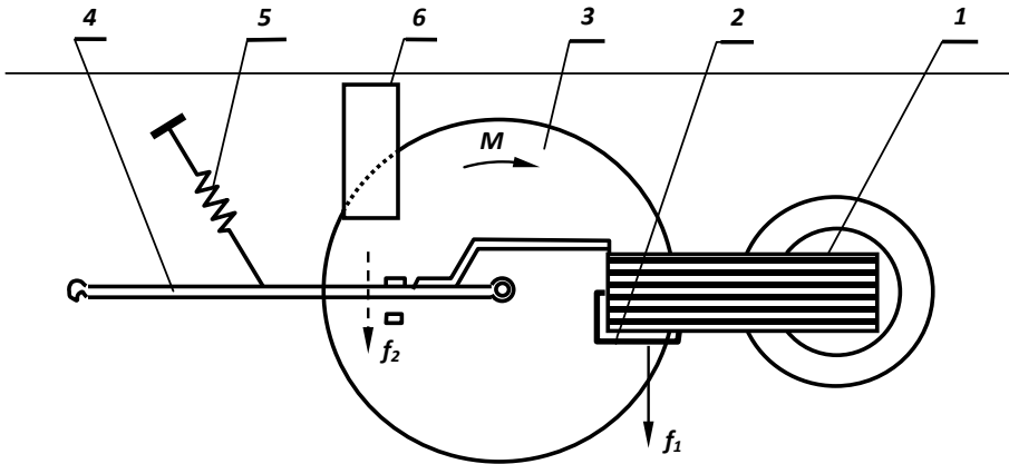
Fig.2.4. Induction disc inverse-type – over-current relay RIz (1-electromagnet, 2-shortcd turn, 3-disc, 4-frame, 5-spring, 6-permanent magnet)
