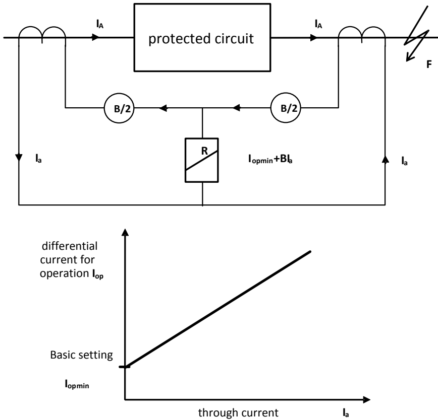
Fig.1.2. Principle of operation of biased differential protection and operating characteristic
