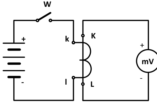
Fig.2.1. Test circuit for the determination of CT terminals
