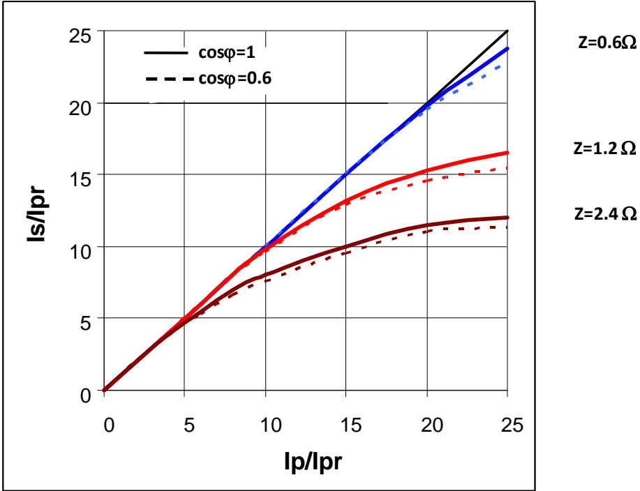
Fig.1.3. Variation of the secondary current I_s value on primary current I_p for different burden value
