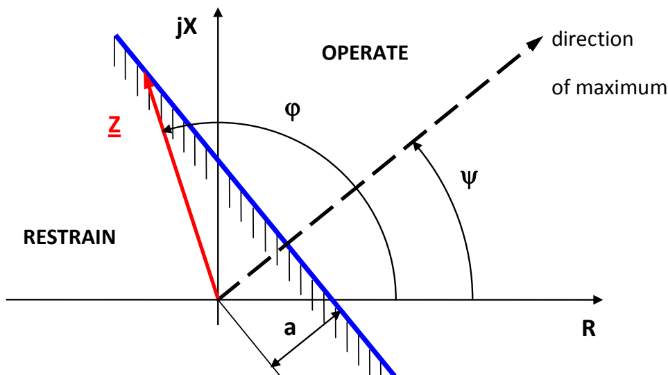
Fig.2.7. Directional relay characteristic on impedance plane
