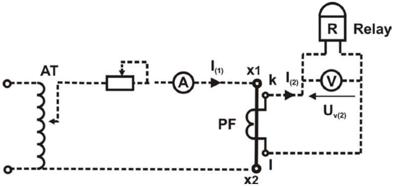
Fig.2.5. Circuit for the current ratio derivation
