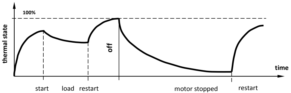
Fig.2.8. Simulated thermal state of a motor
