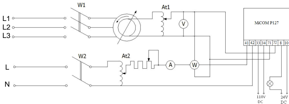
Fig. 3.3. Scheme of connections for testing of MiCOM P127 relay
