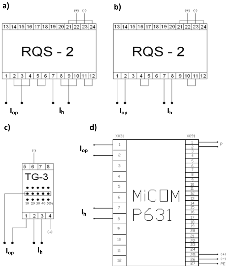
Fig.2.5. Schematic diagram of measuring systems for testing differential relays: a) relay RQS-2 supply of three phases, b) relay RQS-2 (two phases supply), c) relay TG-3, d) relay MICOM P631
