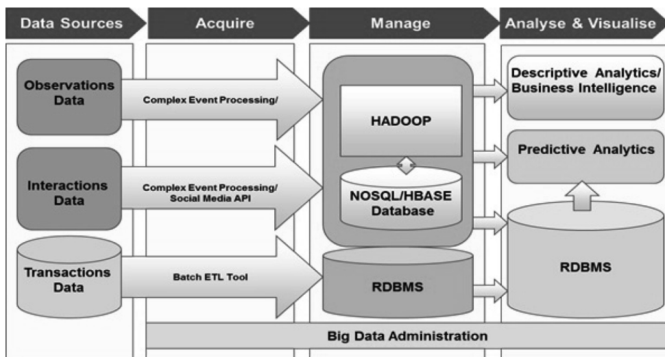
Figure 1. An example of big data architecture
