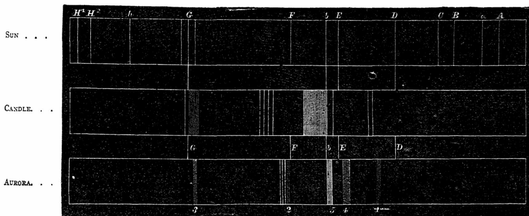
COMPARISON SPECTRA OF SUN, AURORA, AND CANDLE
