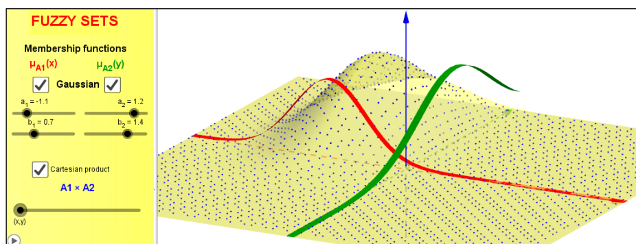
Fig. 6. Cartesian product of fuzzy sets with both Gaussian membership functions in 3D Source: own elaboration.
