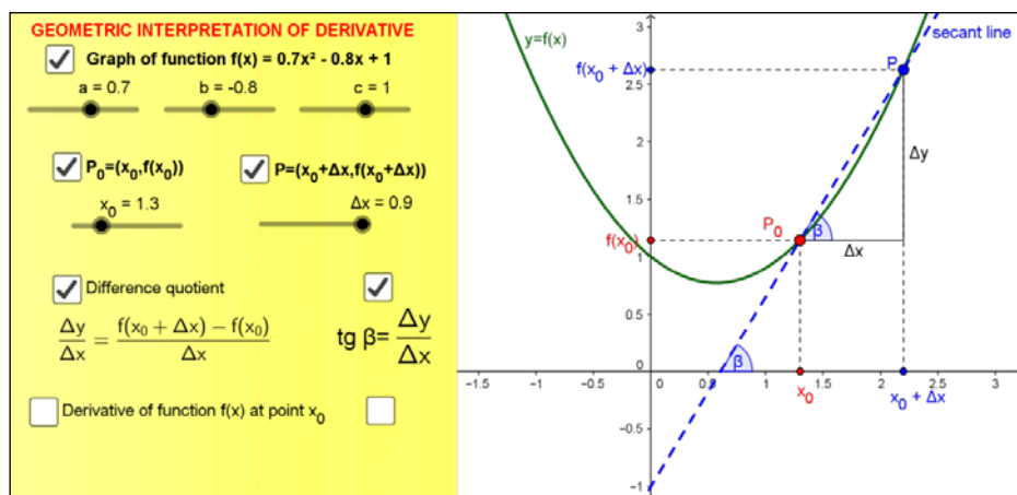
Fig. 8. Difference quotient
