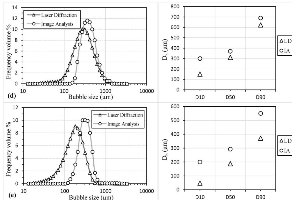
Fig. 9. Results of bubble size measurements using LDT and IAT
