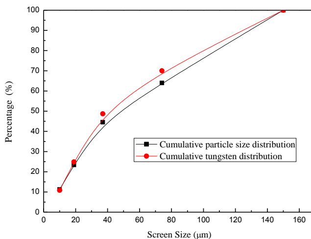
Fig. 1. Cumulative particle size distribution and cumulative tungsten distribution versus particle size
