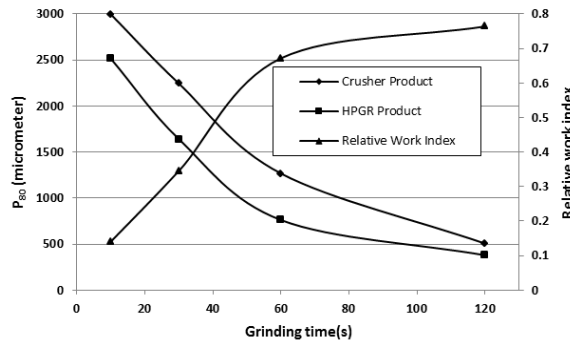
Fig. 8. The variation of HPGR and crusher P_{80} and relative work index \left(\frac{Wi_H}{Wi_C}\right) with grinding time
