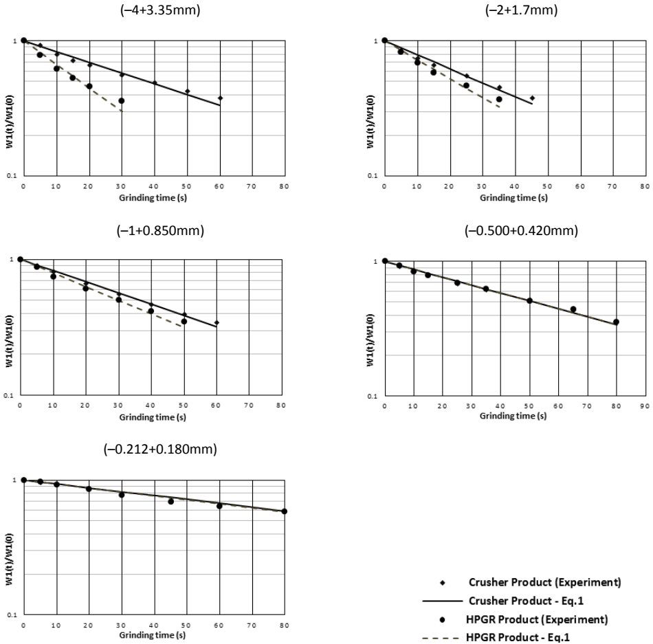
Fig. 5. First-order plot for batch dry grinding of all single sized fractions
