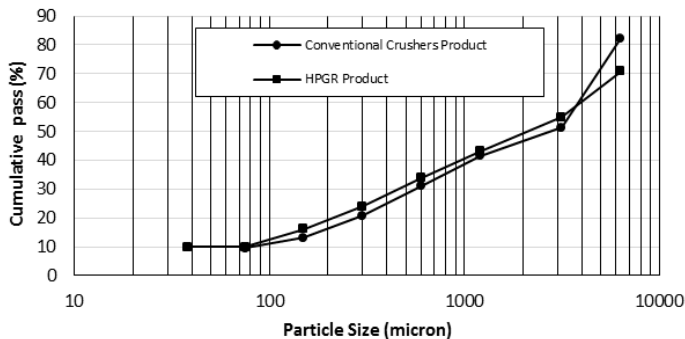
Fig. 2. Particle size distribution of HPGR and conventional crushers
