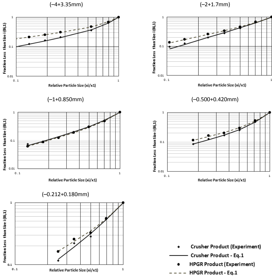
Fig. 4. Cumulative breakage distribution function for all single sized fractions
