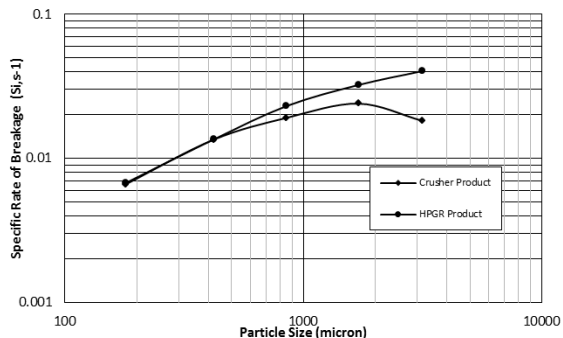
Fig. 6. Specific rates of breakage of ore versus particle size (WSSE, weighted sum squared errors)
