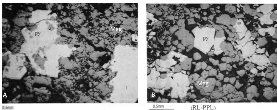
Fig. 3. Inclusions of magnetite in pyrite (A) and gangue mineral enveloped around magnetite grain (B)
