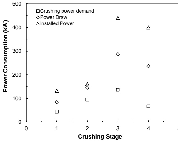
Fig. 10. Three types of power designation
