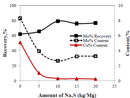
Fig. 6. Effect of Na 2 S on copper and molybdenum flotation (1 kg/Mg Na 2 SiO 3 , 440 g/Mg gas oil, 56 g/Mg pine oil, 58 μm particle size, pH 12)
