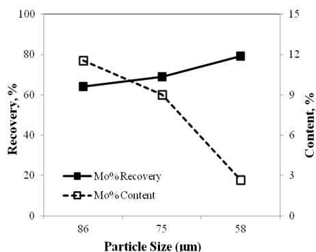
Fig. 4. Effect of particle size on molybdenum flotation (1 kg/Mg \text{Na}_2\text{SiO}_3 , 10 kg/Mg \text{Na}_2\text{S} , 440 g/Mg gas oil, 56 g/Mg pine oil, pH 12)
