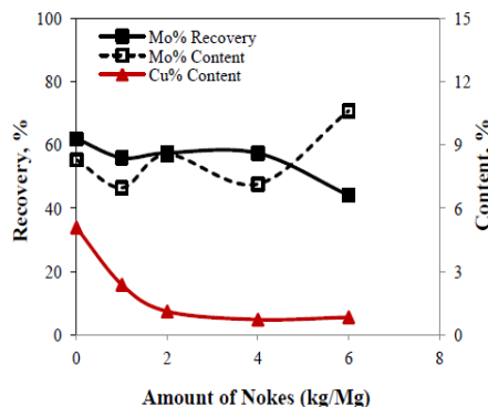
Fig. 7. Effect of Nokes on copper and molybdenum flotation (1 kg/Mg Na 2 SiO 3 , 440 g/Mg gas oil, 56 g/Mg pine oil, 58 μm particle size, pH 12)
