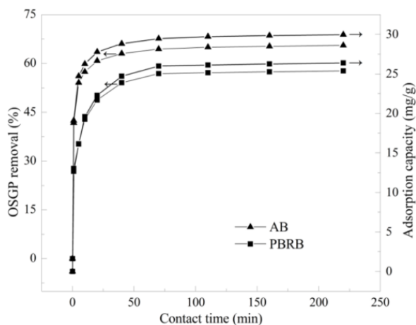
Fig. 8. Effect of contact time on OSGP removal (dose of AB = 35 g/dm 3 , dose of PBRB = 50 g/dm 3 , pigment concentration = 1600 mg/dm 3 , temperature = 298 K)
