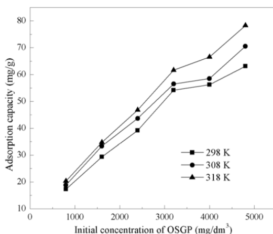
Fig. 9. Effect of initial concentration of OSGP and temperature on amount of adsorbed pigment onto AB (dose of AB = 35 g/dm 3 , contact time = 40 min)
