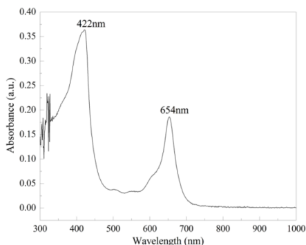
Fig. 2. UV-Vis absorption spectrum of OSGP
