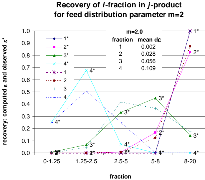
Fig. 6. Results of recovery of i -fraction to the j -product of screening depends on the feed size distribution and distance along classifier chamber: \varepsilon -computed, \varepsilon^* -observed.
