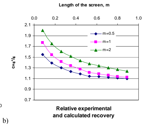
Fig. 5. Nonadditiveness effect of screening depend on feed size distribution and distance from beginning of the screen: \epsilon(L) – recovery predicted, \epsilon(L)^* – observed, c – rate of non-additiveness
