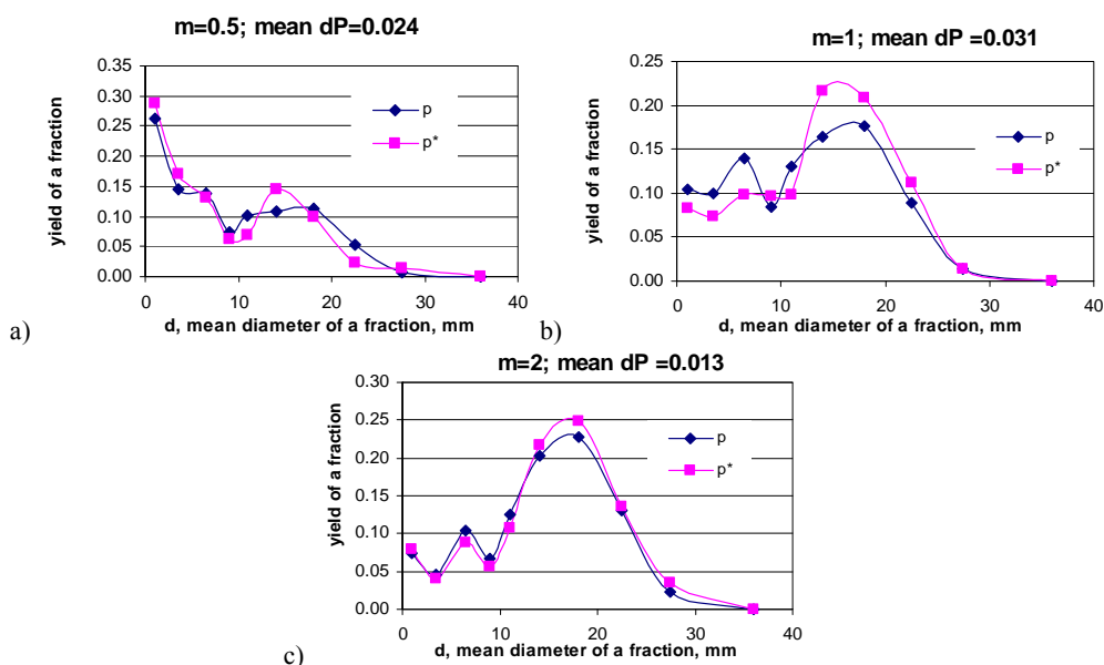
Fig.2. Double-toggle laboratory crusher. Comparison of product size distributions: computed p_k and observed p_k^* for given m_k parameter. Mean dP as in formula (4)
