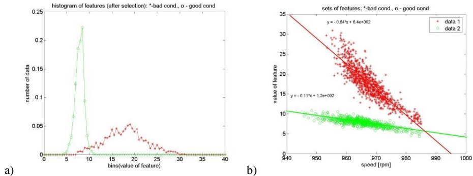
Fig. 10. a) Data distribution of measured diagnostic parameters b) Load susceptibility characteristics as diagnostic features for planetary gearbox as a function of rotation speed RPM; for a gearbox in good (“o” dots) and bad condition (“x” dots)
