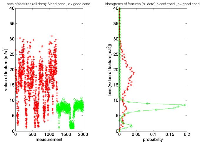
Fig. 9. Probability of feature distributions for two diagnosed objects: circle marked distribution for object in good condition and star marked distribution for object in bad condition
