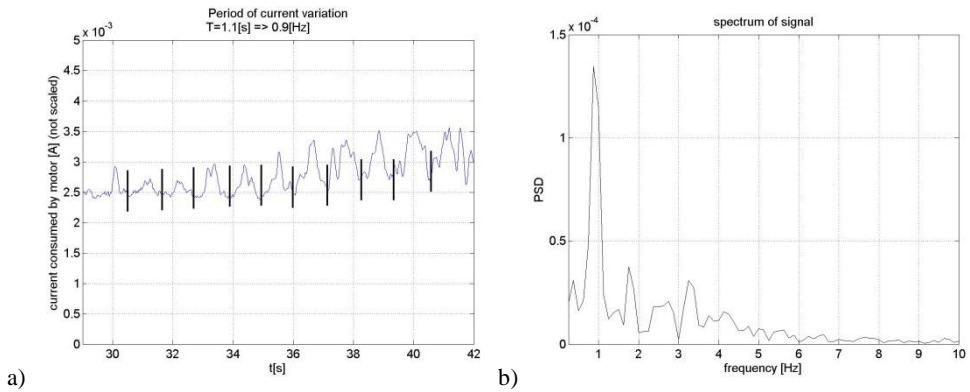
Fig. 3. a) Time fragment of electric current consumption and its spectrum b)
