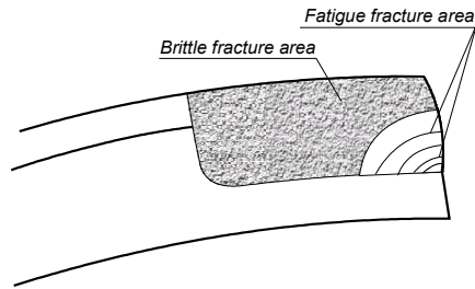
Fig. 7. Scheme of a fatigue fracture area with beach marks and brittle fracture area
