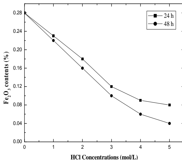
Fig. 5. Iron leaching from silica sand at 25 °C at different concentrations of hydrochloric acid with versus time
