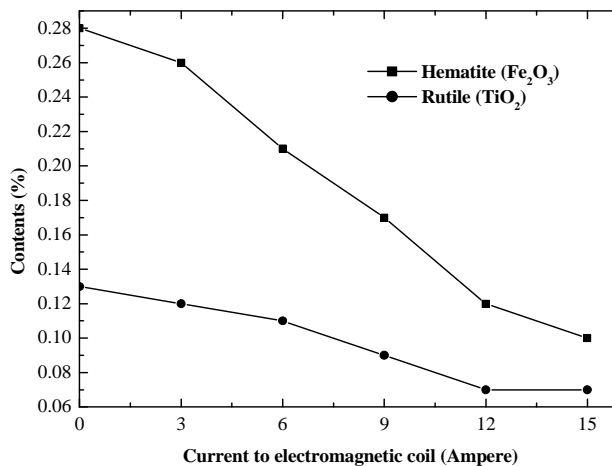
Fig. 4. Effect of current intensity the coil on contents of iron and rutile removal
