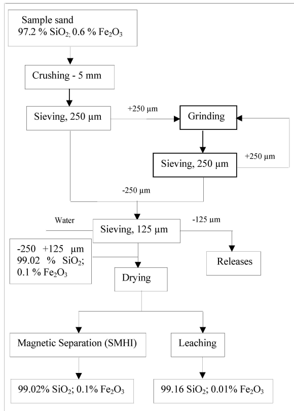
Fig. 7. Flow sheet proposed for the processing of sandstone from El-Aouana deposit
