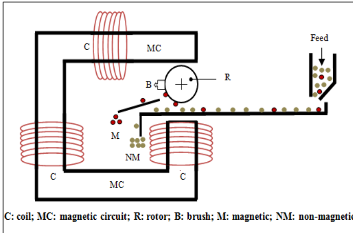
Fig. 1. Magnetic separator high intensity of laboratory (MSHI)
