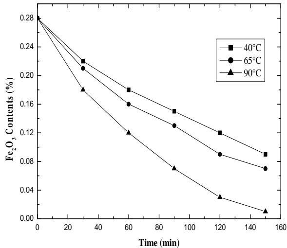
Fig. 6. Iron leaching from silica sand with hydrochloric acid (3 mol/L) versus time at different temperatures
