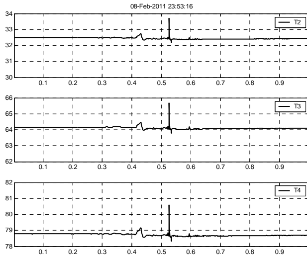
Fig. 5. The recorded dynamic impact on instrumented anchor load variations from a shock with energy level of 5.4 \cdot 10^6 J, at a distance of 188 m from the test position
