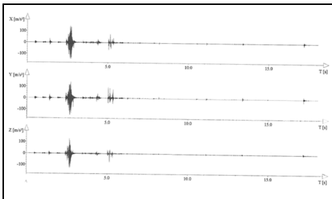
Fig. 4. Diagram of vibration acceleration resulting from a shockwave with an energy level of 5.4 \cdot 10^6 J (epicentre at a distance of 188 m from the test position)
