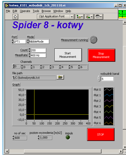
Fig. 2. User's graphic interface of measurement application
