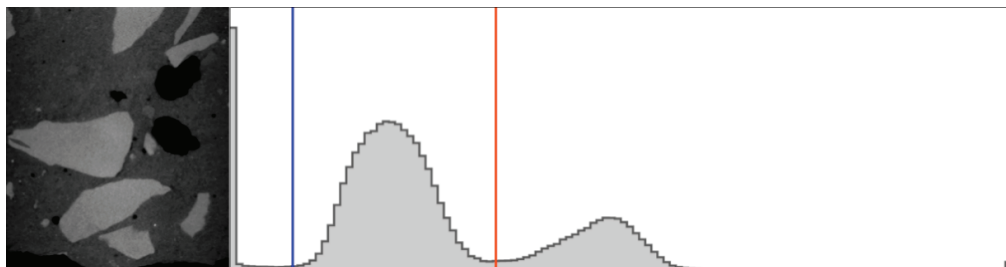
Fig. 7. Image and the corresponding histogram with selected thresholds: blue threshold – pores, red threshold – aggregate
