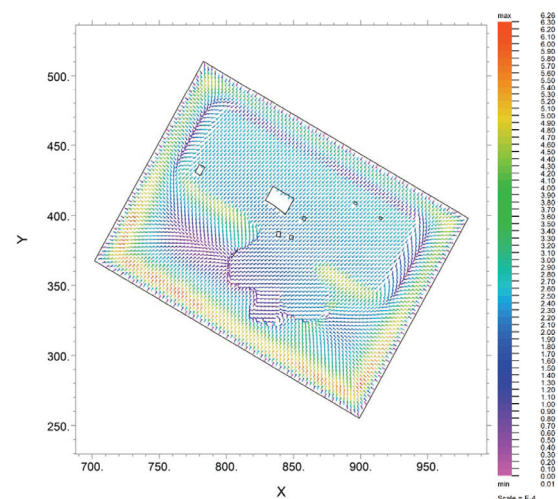
Fig. 11. The vectorial field of horizontal displacements at the top of the foundation slab. (Displacements are expressed in meters; scale multiplier = 1e-4)
