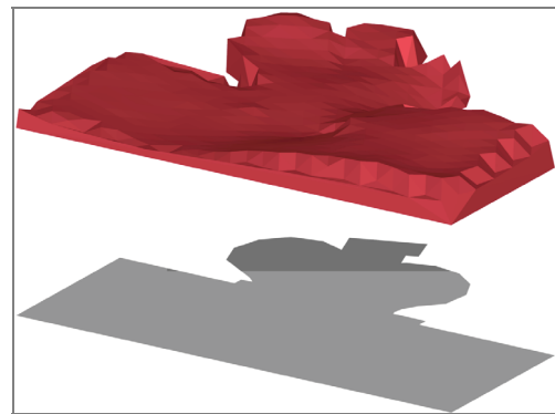
Fig. 10. A spatial image of settlements of the foundation slab
