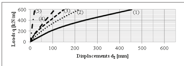
Fig. 4c. Displacements d_2 (mm) depending on the use of sheet piles as a cover of the foundation. Vertical load applied at the bearing points
