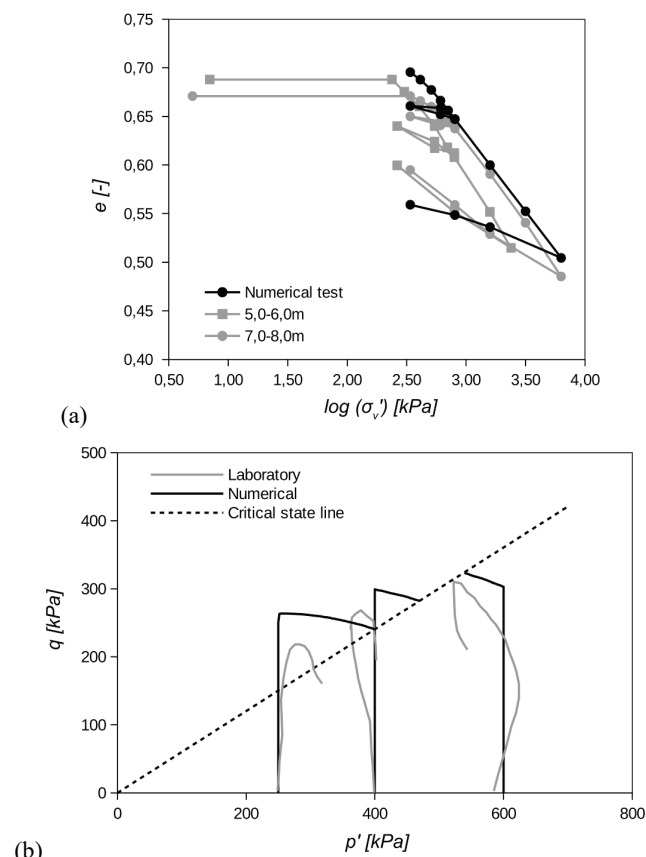
Fig. 3. Calibration of geotechnical parameters: (a) oedometer test, (b) triaxial test
