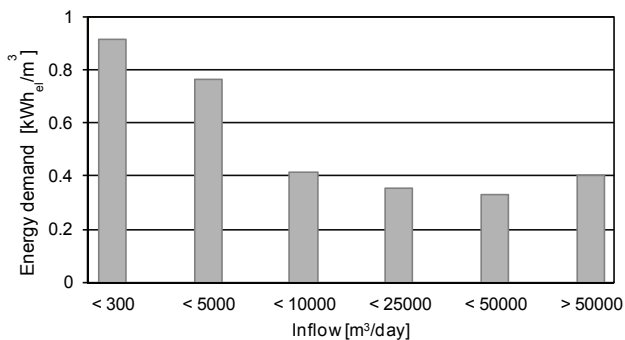
Fig. 3. Specific energy demand by daily inflow groups-
