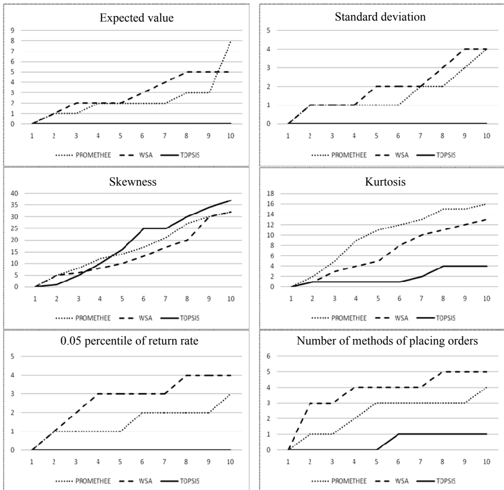
Fig. 3. Values of the s measure in consecutive iterations for the first group of criteria and the number of methods of placing orders criterion (decreasing weights).
