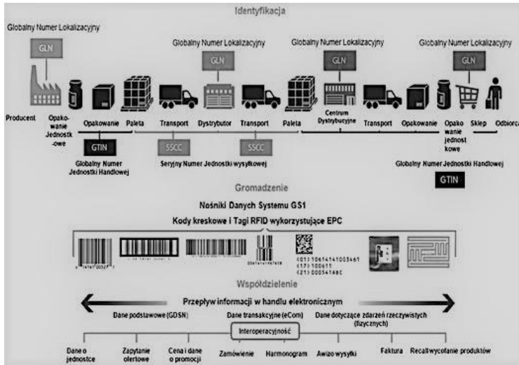
Rys. 6. System GS1
