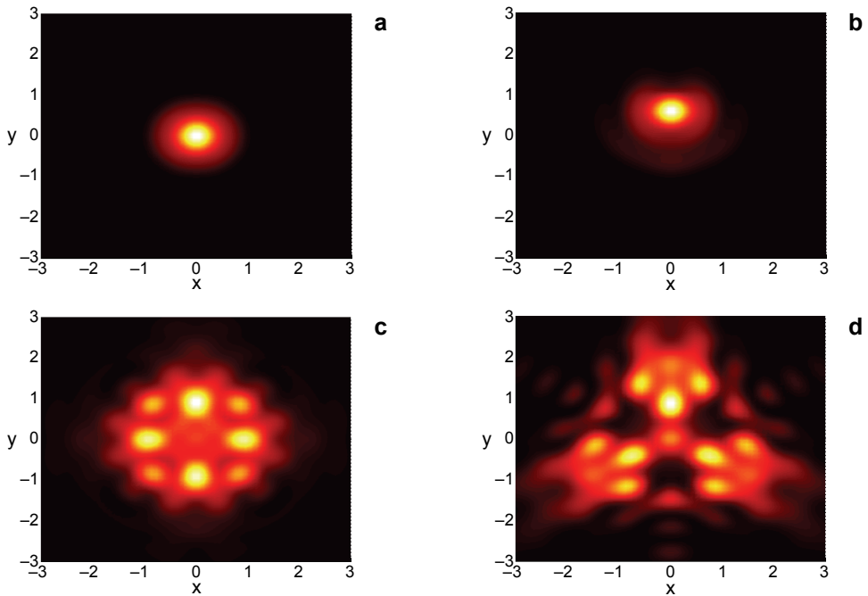
Fig. 8. Intensity distributions for \beta_1 = 1 , NA = 0.95 , and m = 0 (a), m = 1 (b), m = 2 (c), m = 3 (d).
