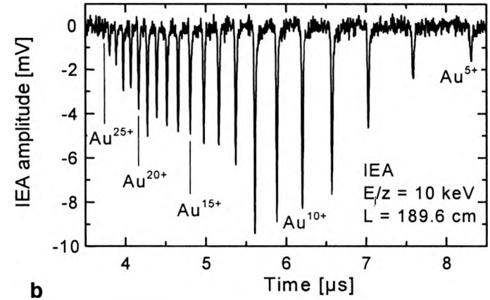
Fig. 2. IC1 collector signals (top) and IEA spectra (bottom) of Au ions for the ps (a) and the sub-ns (b) laser pulses.
