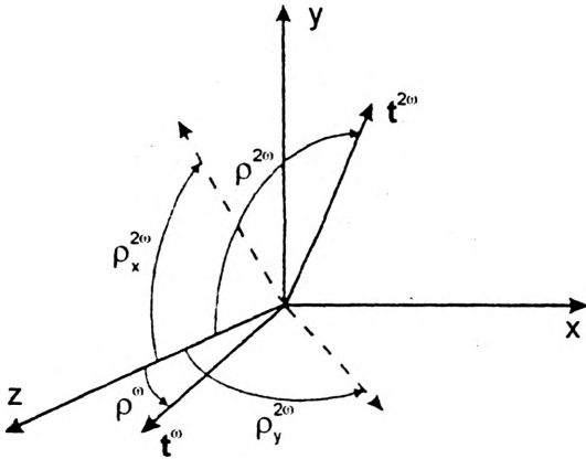
Fig. 1. Orthogonal phase-matching system x||\mathbf{D}^\omega , y||\mathbf{D}^{2\omega} and z||s of the MBANP molecular crystal. The propagation of the waves at both frequencies is in the z -direction. The angle \rho^\omega is the beam walk-off of the fundamental beam with the Poynting vector \mathbf{t}^\omega propagating in the (x, z) plane. Direction of the second-harmonic Poynting vector is denoted by \mathbf{t}^{2\omega} and its beam walk-off angle by \rho^{2\omega} . The projections of this angle onto (y, z) and (x, z) are denoted by \rho_x^{2\omega} and \rho_y^{2\omega} , respectively. For clarity, the angles are shown in enormous proportions.
