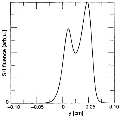
▲ Fig. 3. Projection of the second-harmonic beam onto the (y, z) plane of the phase-matching system.
